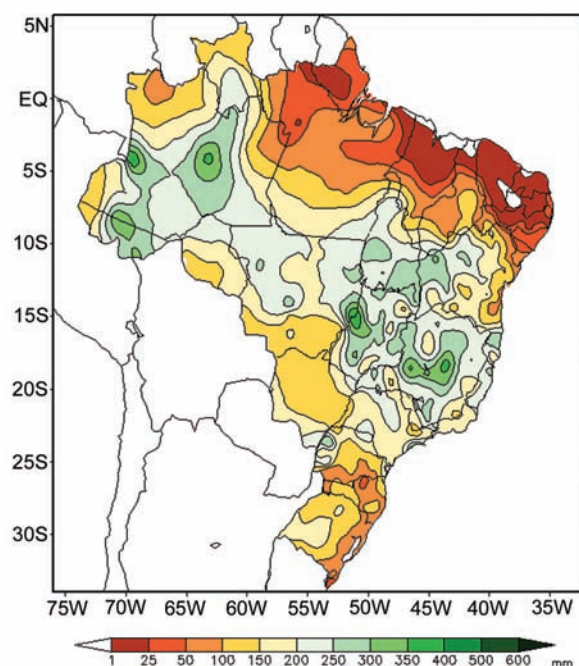
Figure 6.1. Contour map of precipitation
