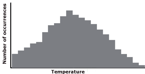
Figure 4.1. Frequency distribution (histogram)
