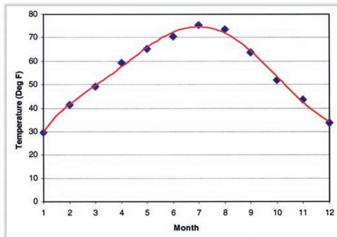
Figure 6.14. Line graph of a time series emphasizing observed values
