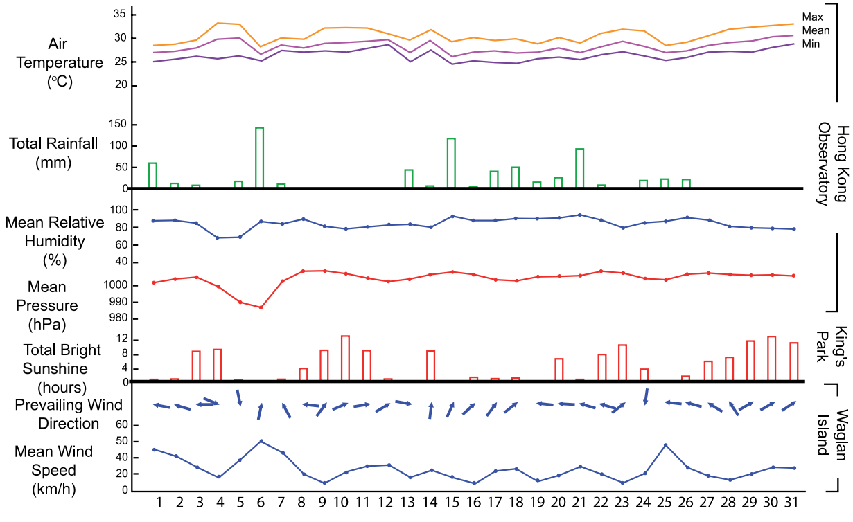
Figure 6.2. Graphical display of daily values of several elements
