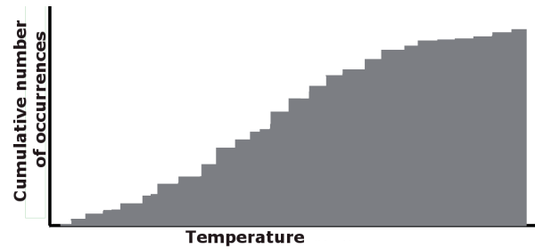
Figure 4.2. Cumulative frequency distribution
