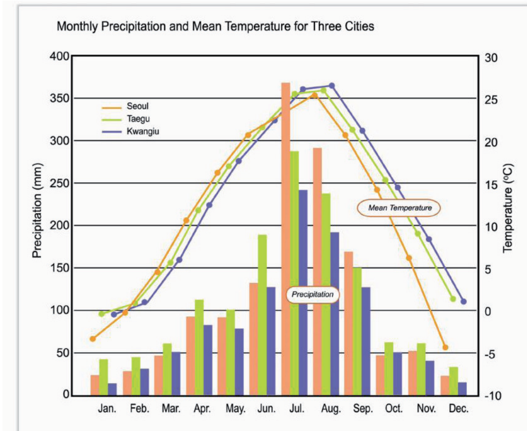
Figure 6.9. Composite line and bar chart for multiple elements and stations
