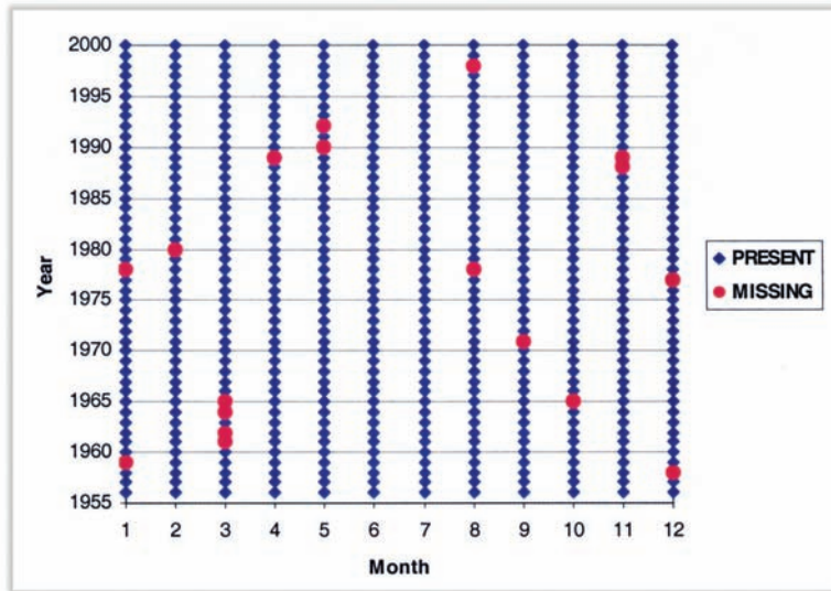
Figure 6.10. Visual display of months with complete and missing data
