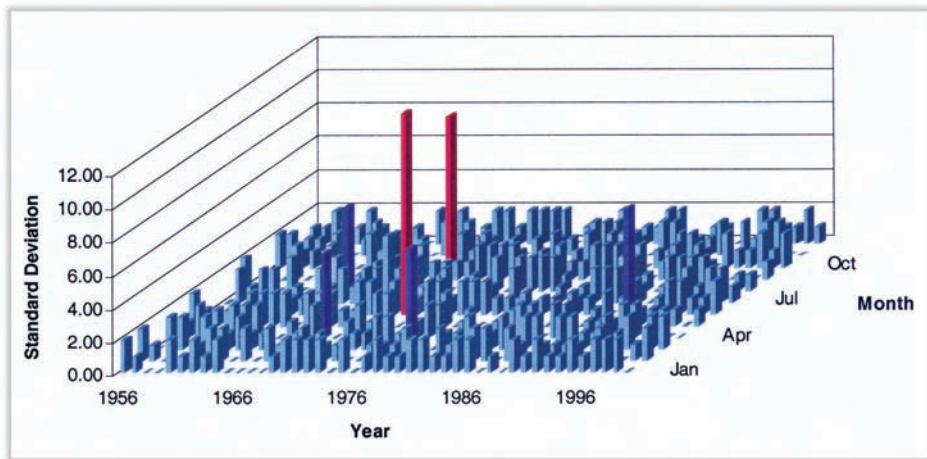
Figure 6.11. Three-dimensional display emphasizing anomalous values
