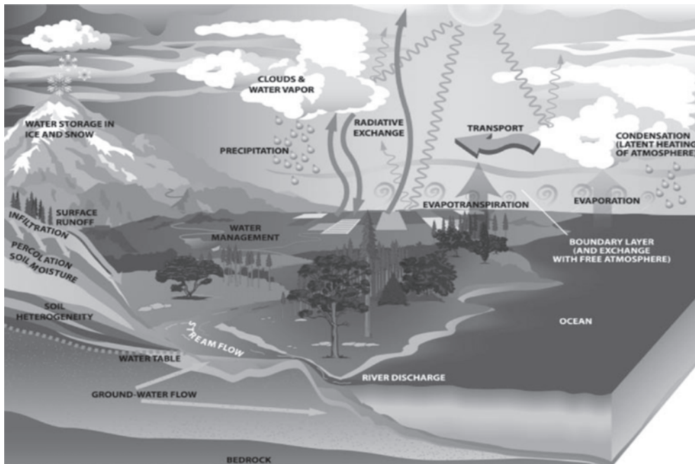
Figure 1.1. The climate system
