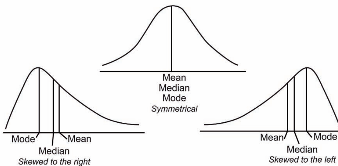
Figure 4.15. Relationships among the mean, median and mode
