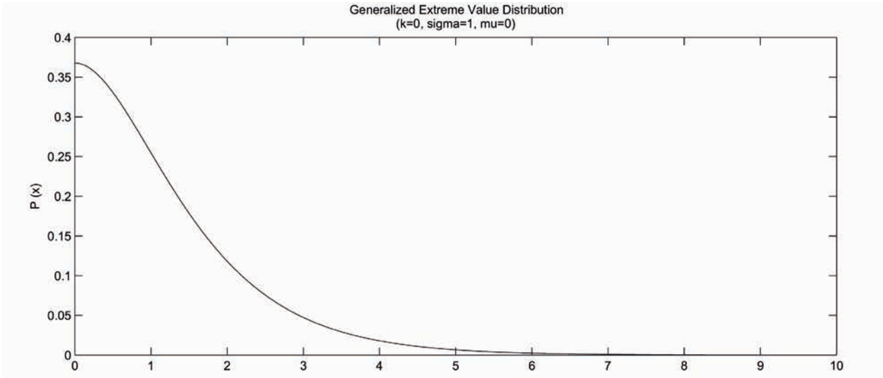
Figure 4.9. Generalized extreme value distribution: Used to model extreme values in a distribution.
