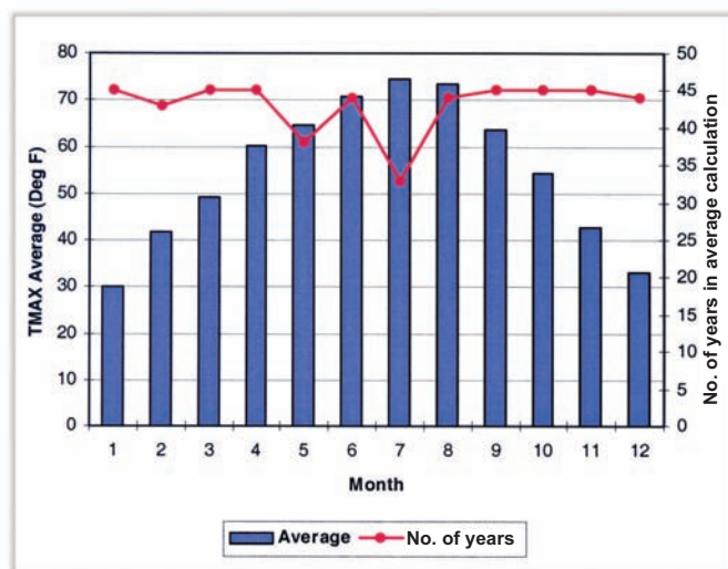
Figure 6.15. Composite bar chart and line graph of average temperature values and number of years of record
