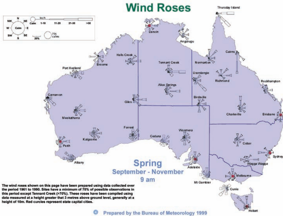
Figure 6.17. Symbolic map display of wind
