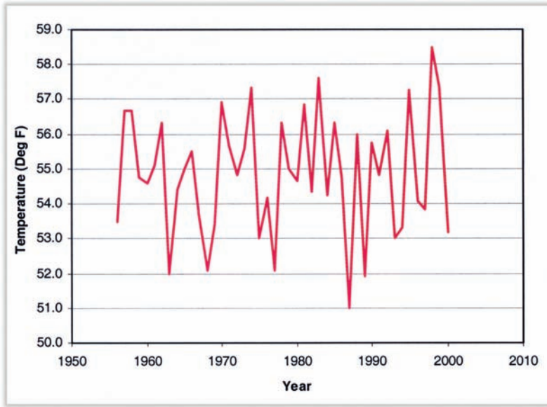
Figure 6.13 Line graph of a time series
