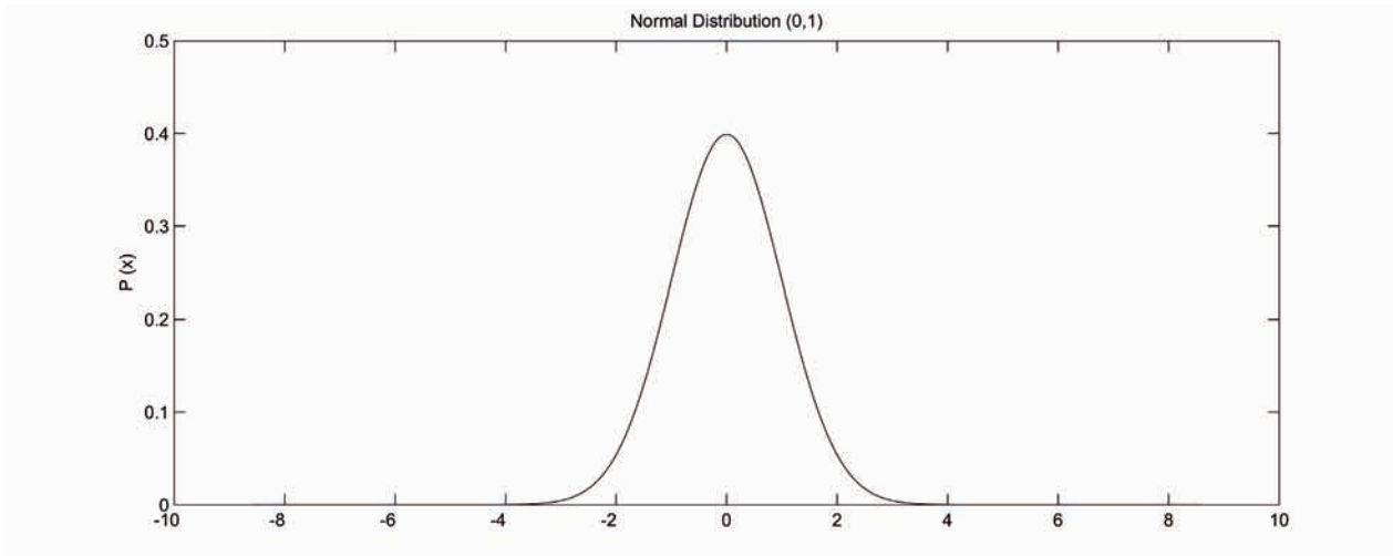
Figure 4.6. Normal or Gaussian distribution: Values over the range for the property being observed tend to cluster uniformly around a single value, such as annual average temperatures.
