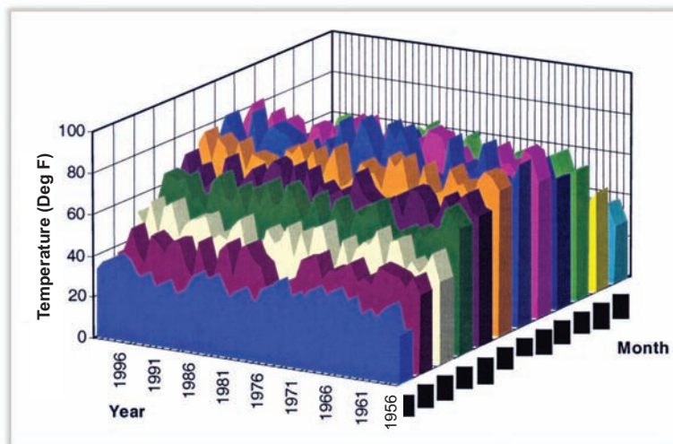
Figure 6.12. Three-dimensional display emphasizing time series of monthly values for a given year
