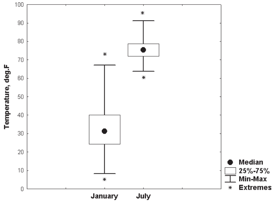
Figure 4.3. Box plot
