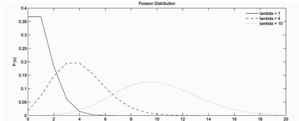
Figure 4.14. Poisson distribution: Describes rare events, such as the frequency of occurrence of tropical storms.
