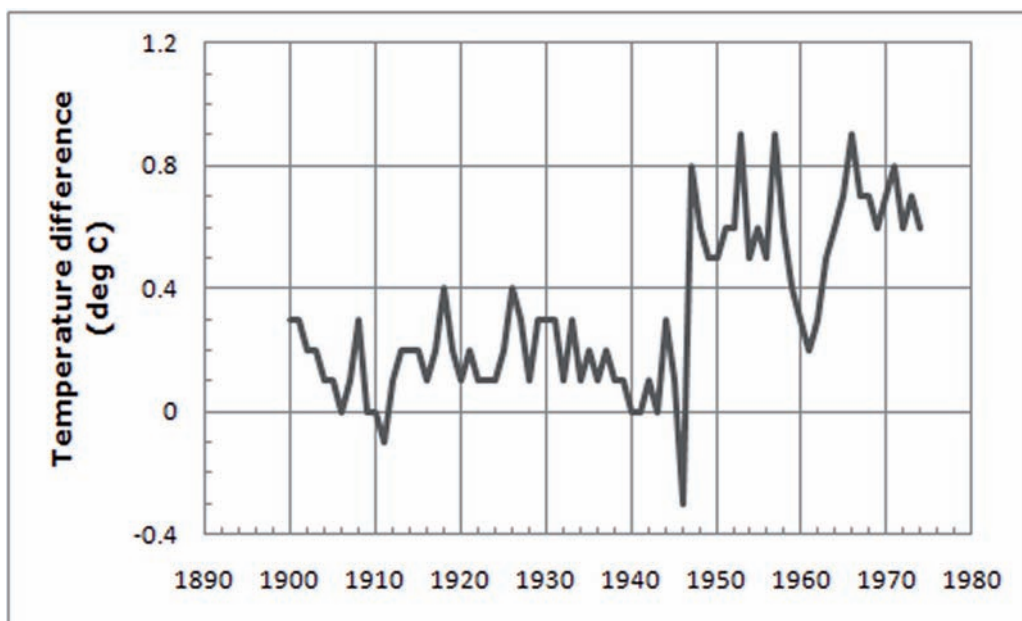
Figure 5.2. Example of a difference time series
