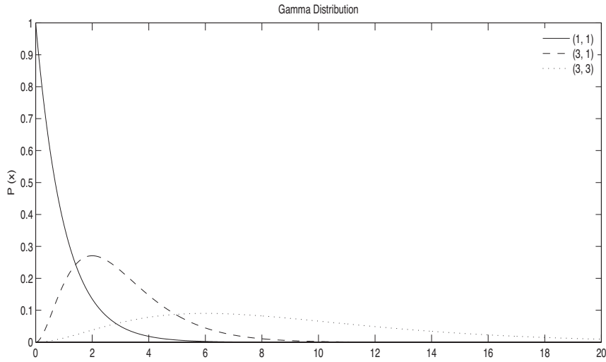
Figure 4.11. Gamma distribution: Describes distributions that are bounded at one end and skewed, such as precipitation data.
