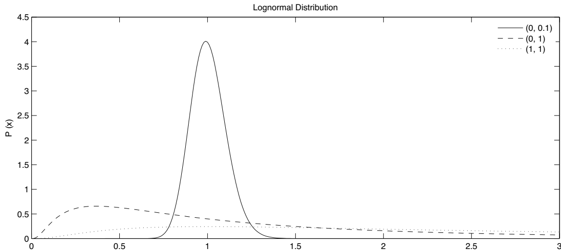
Figure 4.10. Lognormal distribution: Used when the logarithm of a distribution follows the normal distribution, such as the distribution of air pollution particle concentrations.
