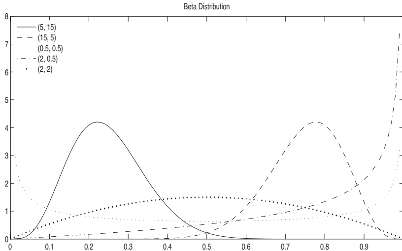
Figure 4.12. Beta distribution: Describes distributions that are bounded at both ends, such as cloud amounts.
