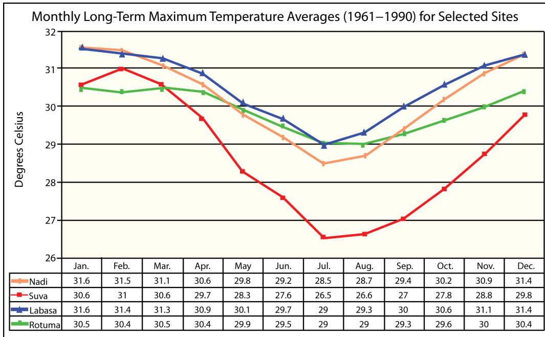
Figure 6.4. Line graph and table of temperature values for multiple stations
