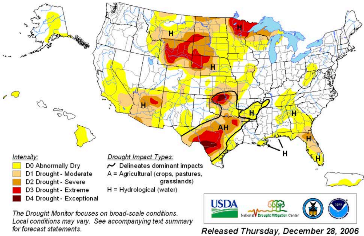
Figure 6.16. Contour map of drought categories and impacts
