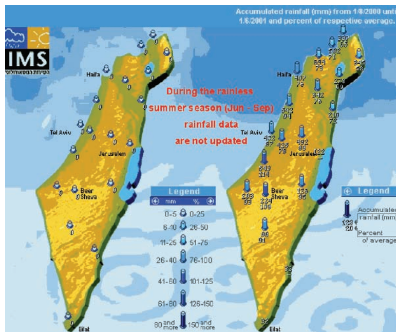
Figure 6.7. Symbolic map display of rainfall information
