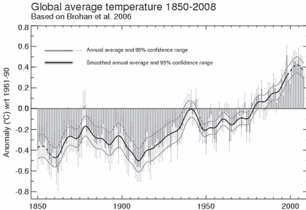
Figure 4.19. Global average temperature anomalies (courtesy Met Office Hadley Centre, United Kingdom)
