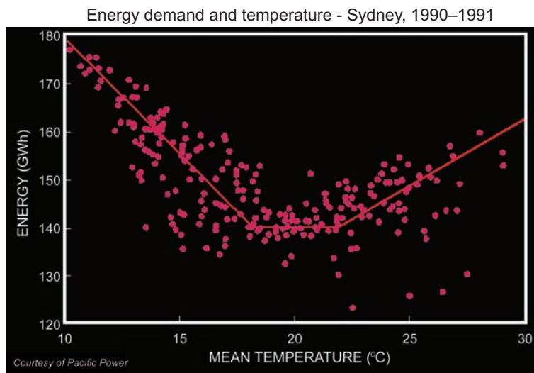
Figure 6.3. Scatter diagram of energy demand and temperature with trend line superimposed
