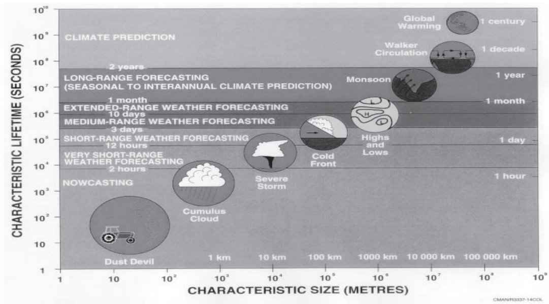
Figure 1.3. Lifetime of atmospheric phenomena (after J.W. Zillman, WMO Bulletin , Vol. 48(2), 1999)
