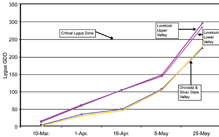
Figure 6.5. Graphical display of growing degree-days throughout a season for multiple stations
