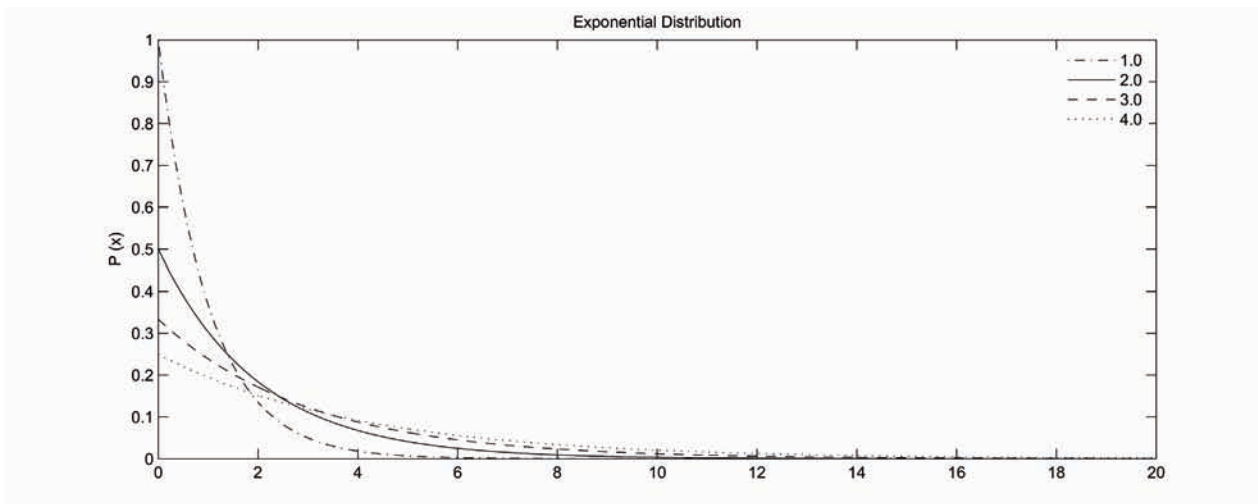
Figure 4.7. Exponential distribution: Describes the times between events in a process in which events occur continuously and independently at a constant average rate and has been used in daily precipitation amount analyses.
