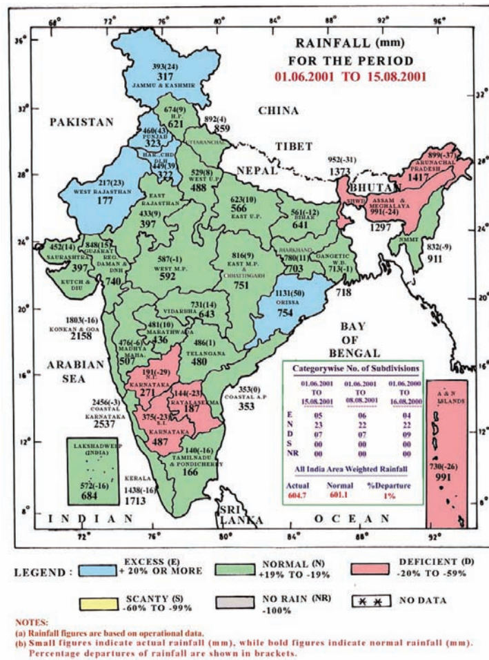
Figure 6.6. Map of regional values of rainfall with a table of summary information
