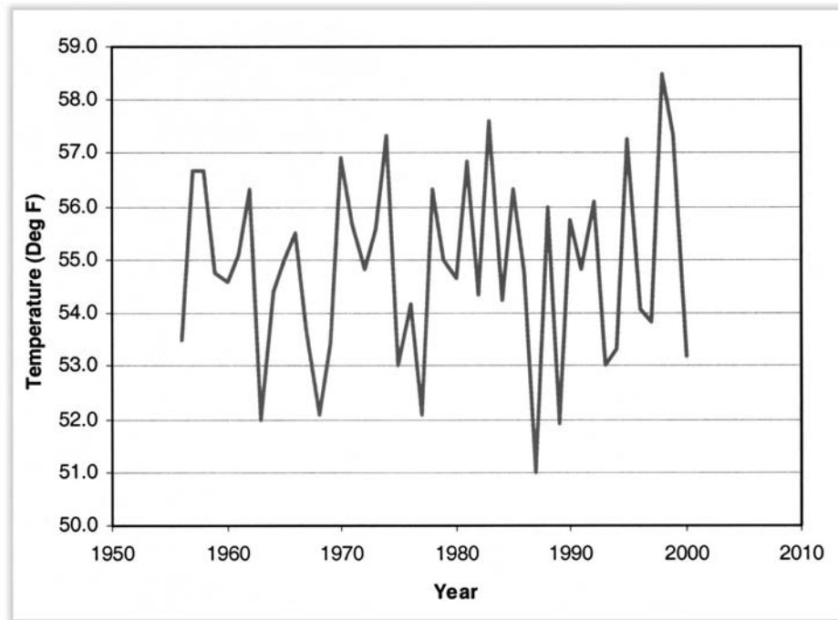
Figure 4.18. Time series of monthly average temperature
