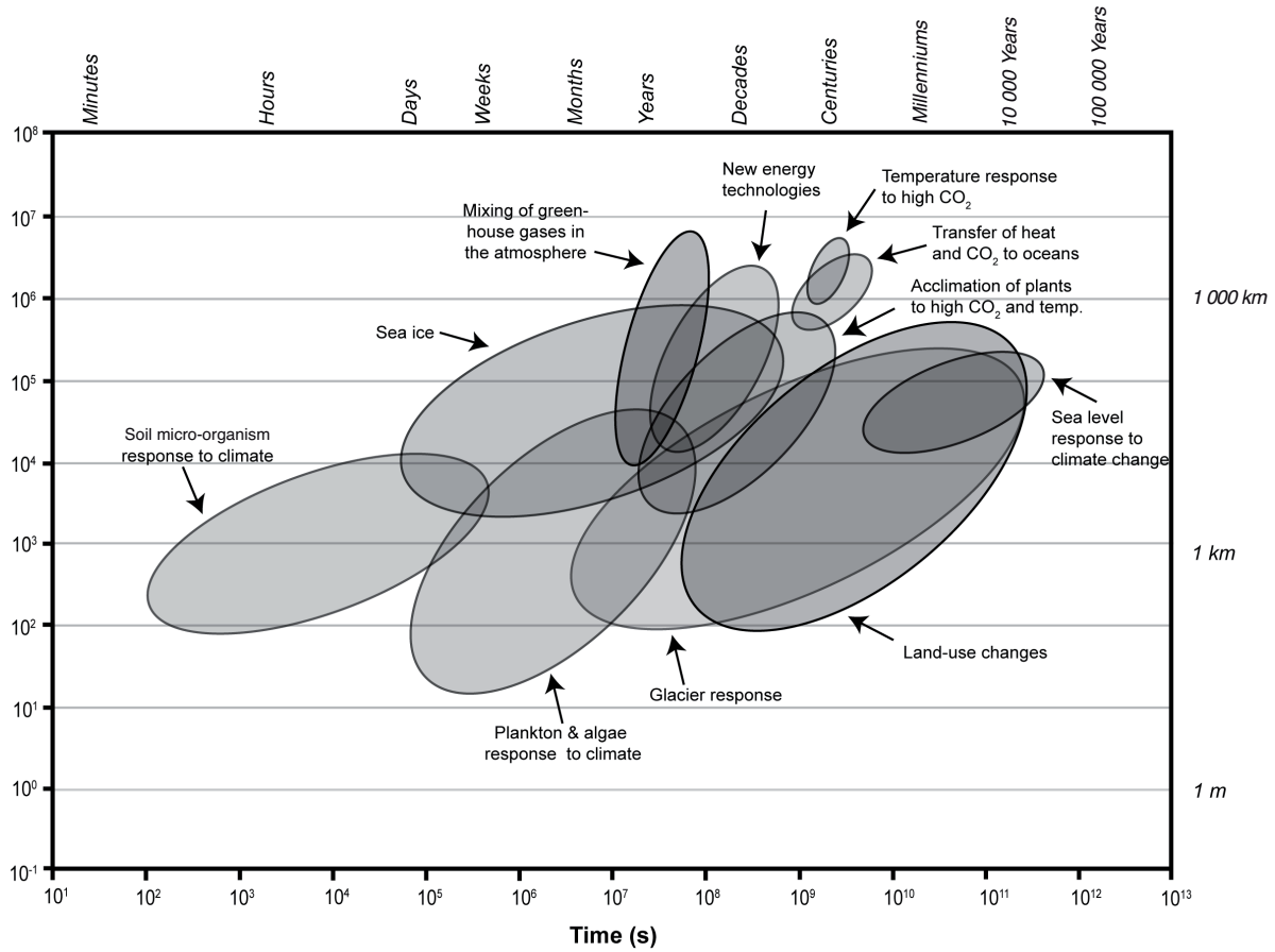
Figure 1.2. Temporal and spatial scales (courtesy Todd Albert, United States)
