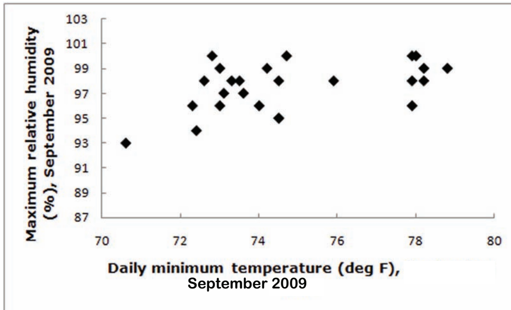
Figure 4.17. Scatter diagram with strong positive correlation
