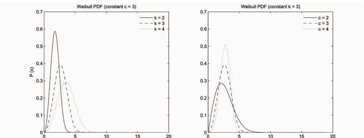
Figure 4.8. Weibull distribution: Describes the times between events in a process in which events occur continuously and independently at a varying rate and has been used in wind speed analyses.
