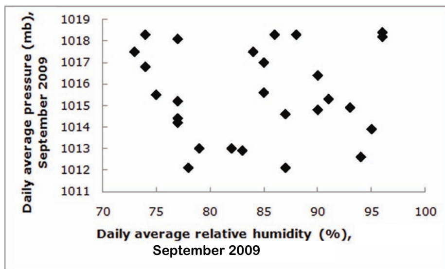
Figure 4.16. Scatter diagram with weak correlation
