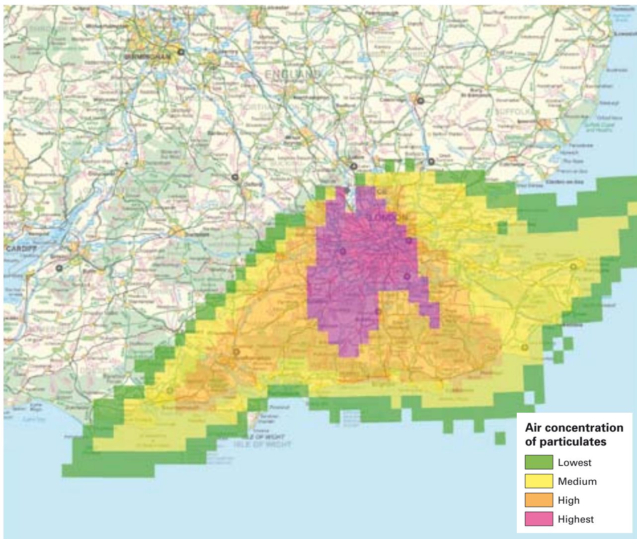
The dispersion model mapping the density of the plume across the south-east of the UK from the Buncefield fire, 2005 8
