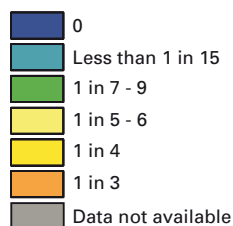
Drought frequency in number of years (yrs)
