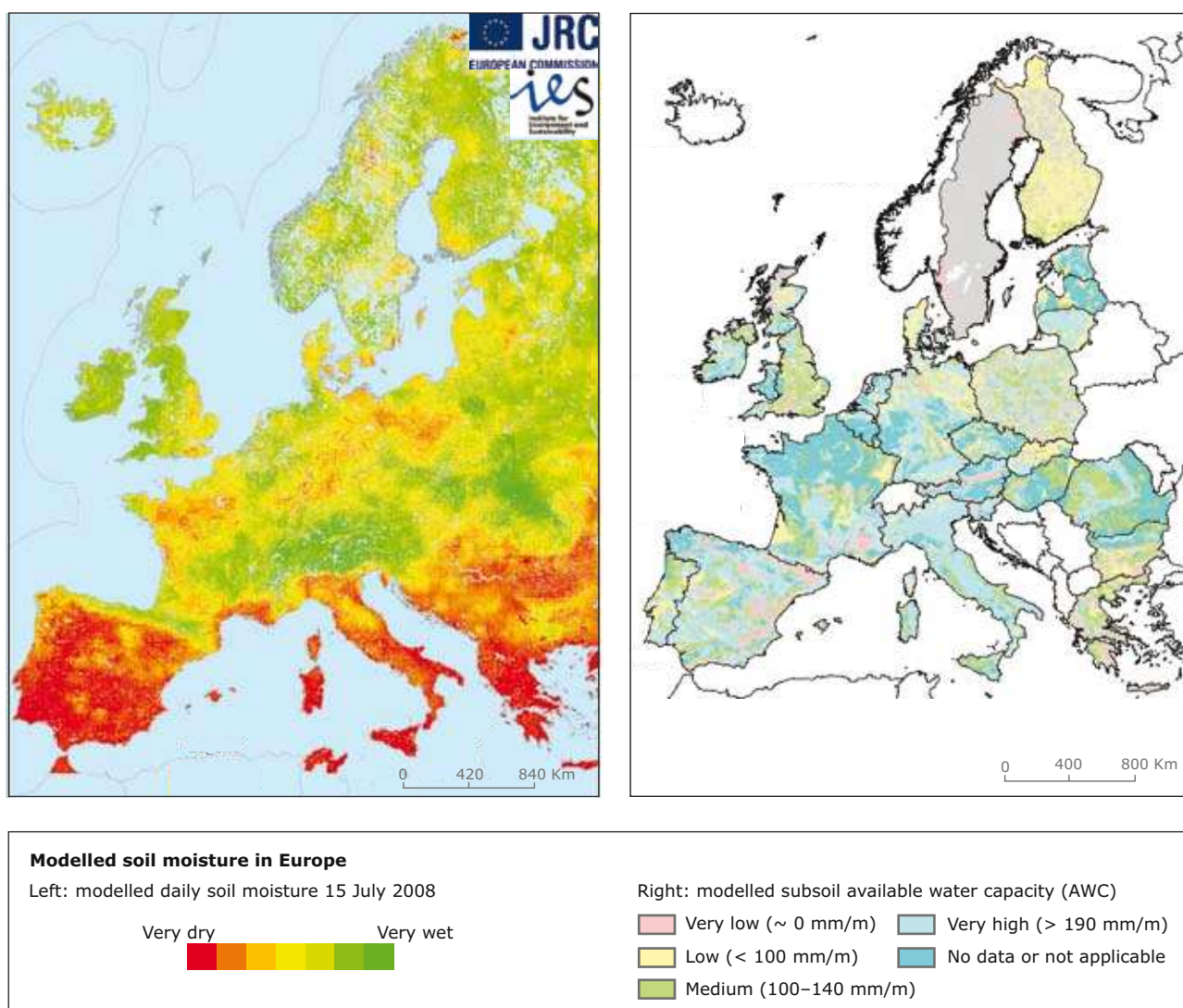
Map 5.38 Modelled soil moisture in Europe
