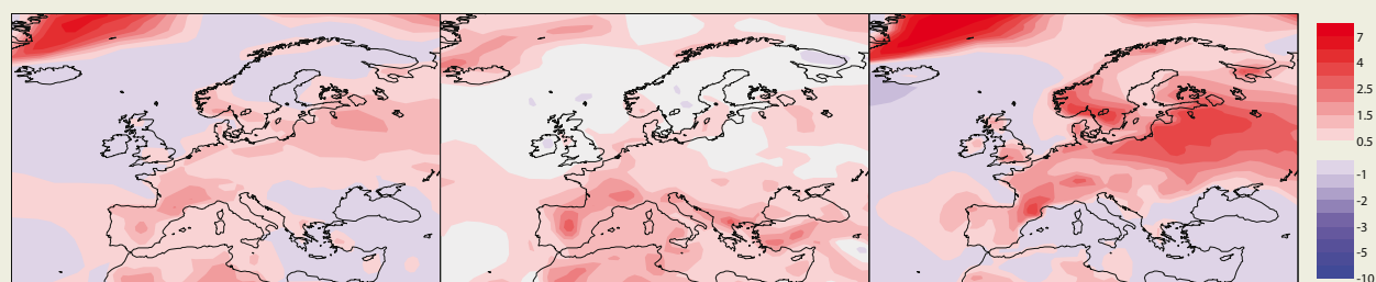
Map 5.3 The linear trend in surface temperature over Europe 1958–2001
