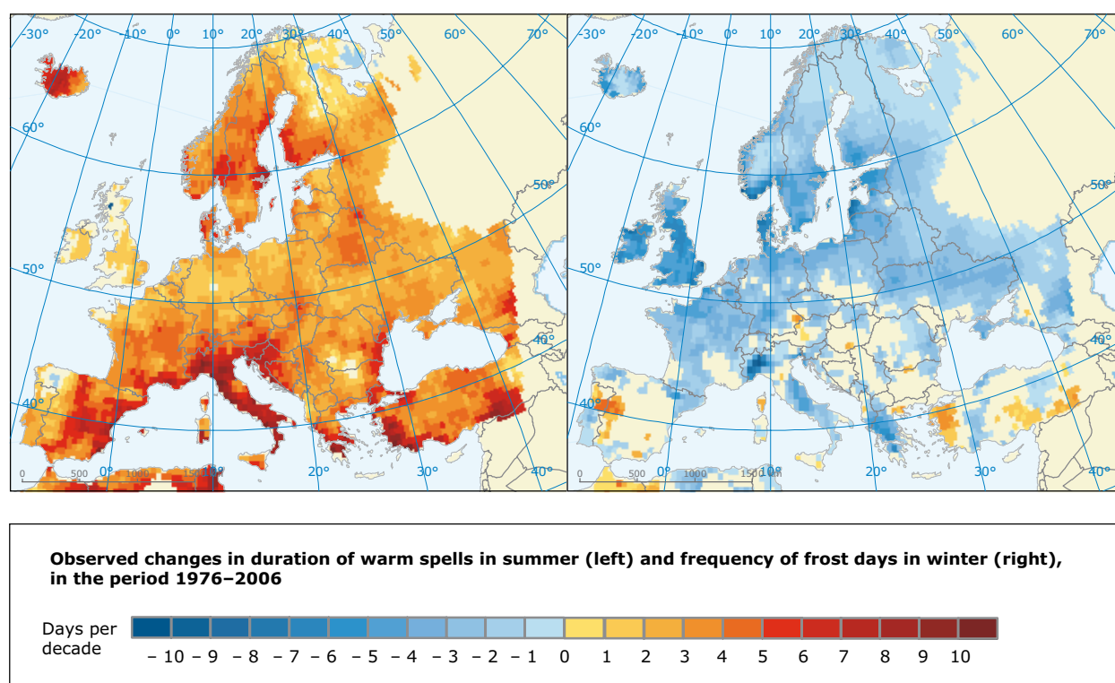
Map 5.6 Observed changes in warm spells and frost days indices 1976–2006
