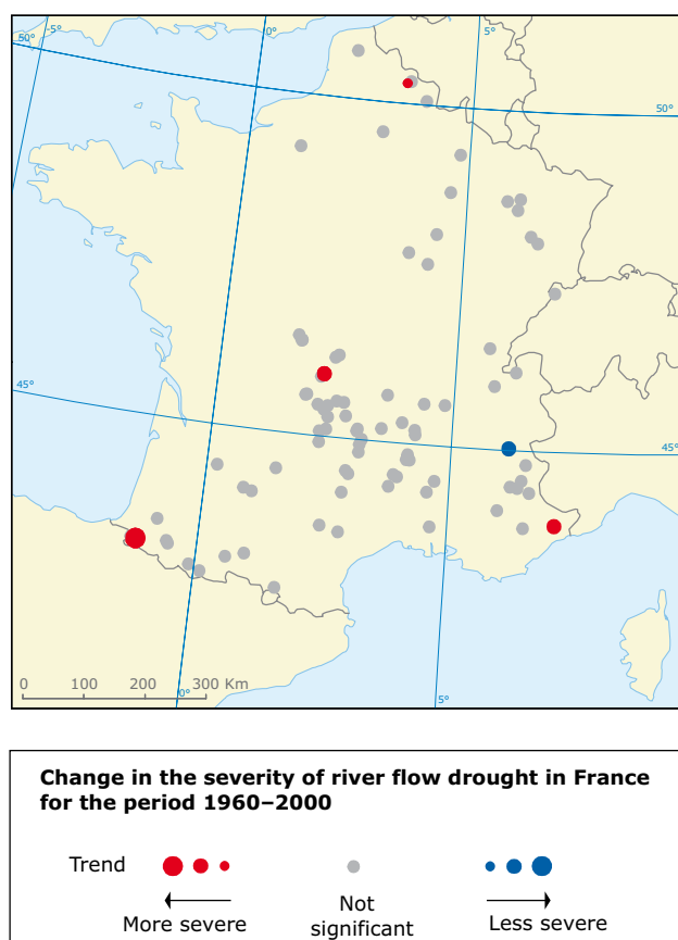
Map 5.27 Change in the severity of river flow droughts in France 1960–2000
