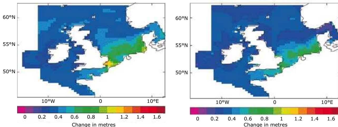
Map 5.11 Change in the height of a 50-year return period extreme water level event for the end of 21st century for different scenarios
