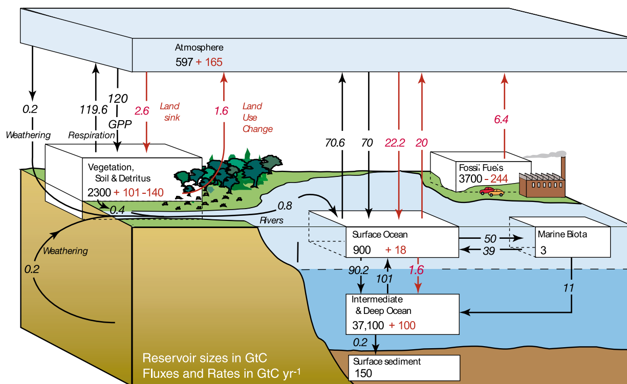
Figure 2.2 The global carbon cycle for the 1990s
