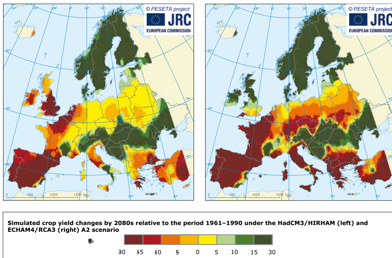
Map 7.4 Projected crop yield changes between the 2080s and the reference period 1961–1990 by two different models
