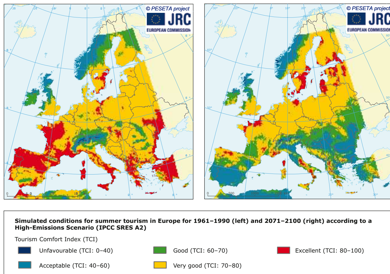
Map 7.6 Modelled conditions for summer tourism in Europe for 1961–1990 and 2071–2100
