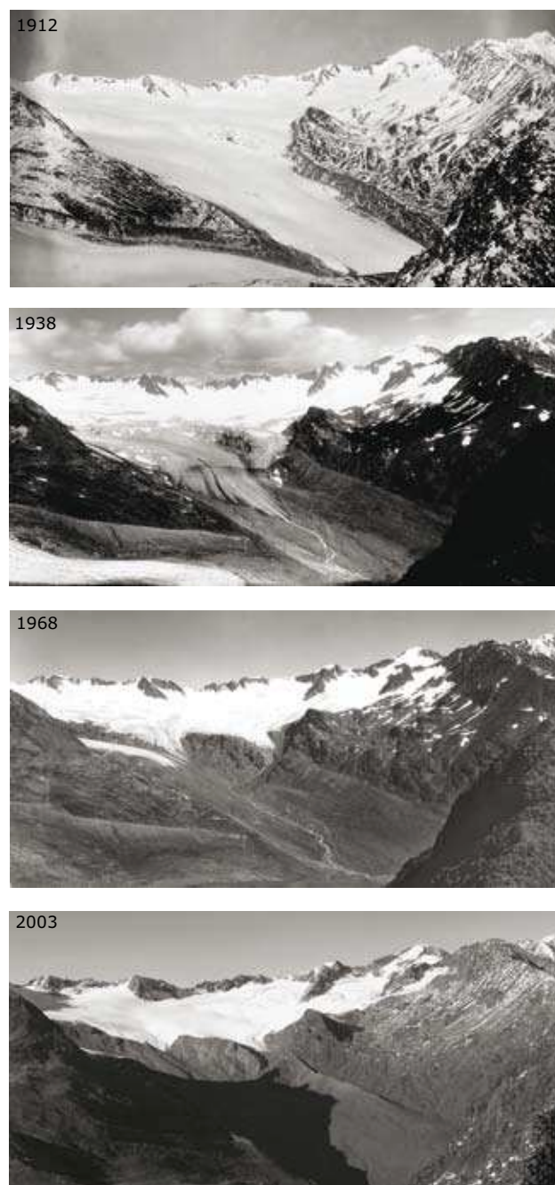
Figure 5.9 Shrinking of the Vernagtferner glacier, Austria
