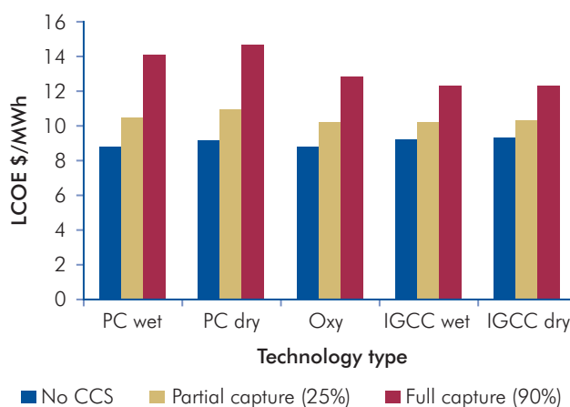
Figure 6.1: LCOE for Reference Plants without CCS and Plants with CCS for the Five Technologies Examined
