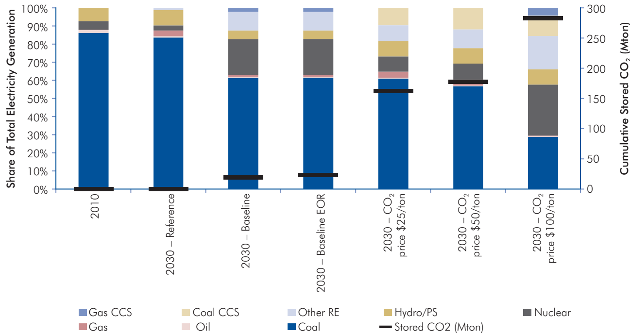
Figure 3.5: Summary of Results for Southern African Region, 2030
