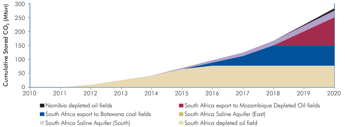
Figure 3.4: Cumulative CO 2 Storage for Southern African Region—US$100/Ton CO 2 Scenario
