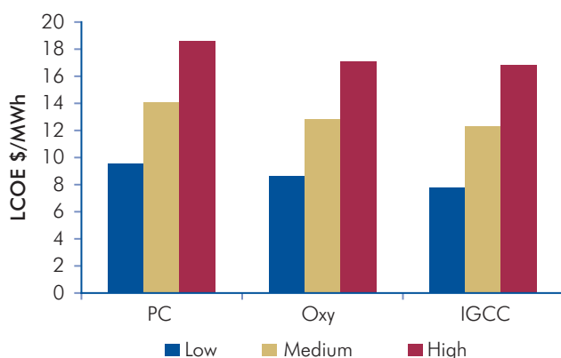
Figure 6.2: LCOE for Full Capture Coal Plants with CCS with Different Coal Prices
