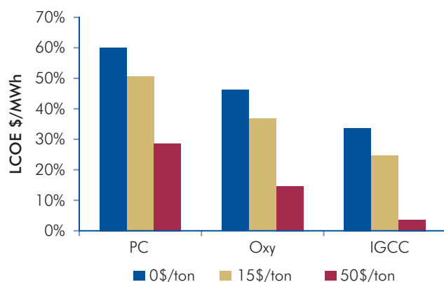
Figure 6.4: Percentage Increase in LCOE from Reference Plant to Plant with CCS for Different CO 2 Prices
