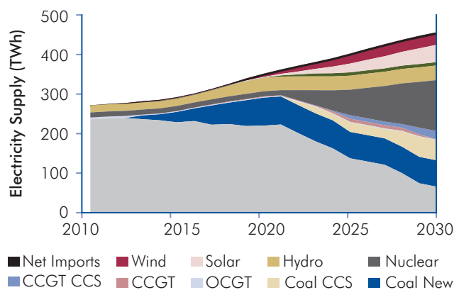
Figure 3.3: Electricity Generation Portfolio for Southern African Region—US$100/Ton CO 2 Price Scenario
