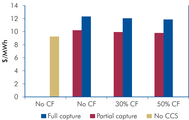
Figure 6.7: LCOE with Different Levels of Concessional Financing for IGCC plant
