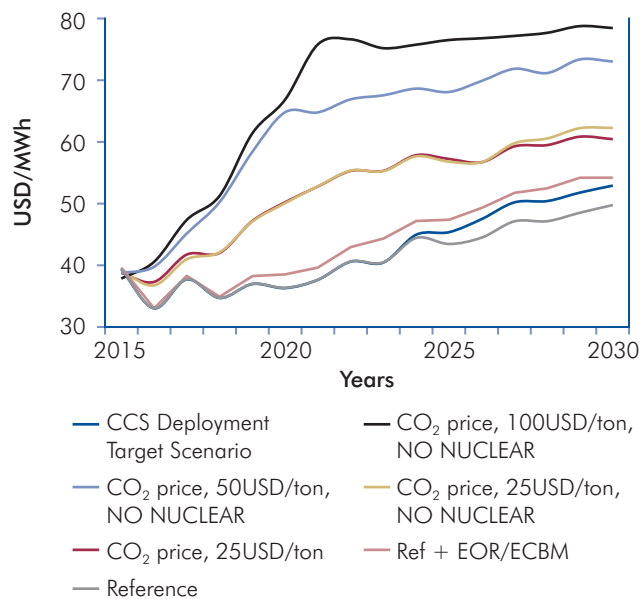
Figure 3.14: Comparison of Average Generation Costs across Scenarios for the Balkan Region
