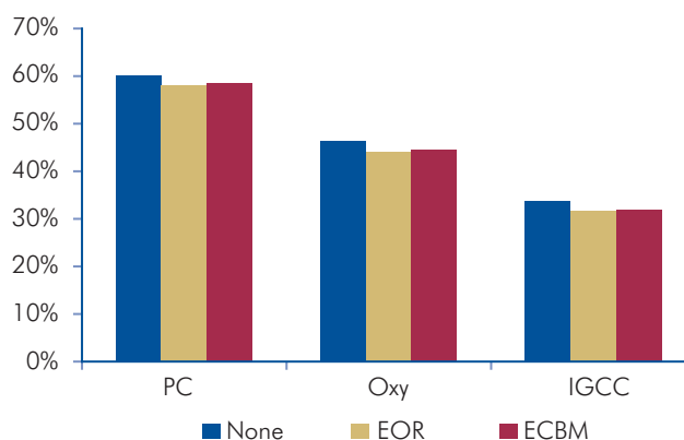
Figure 6.5: Percentage Increase in LCOE for a Reference Plant without CCS to a Plant with CCS and Enhanced Hydrocarbon Recovery
