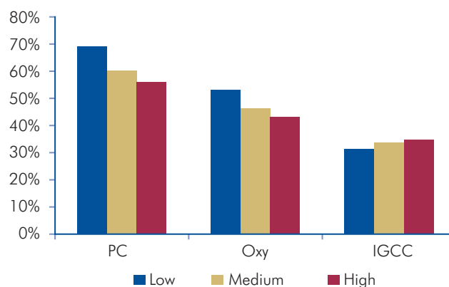
Figure 6.3: Percentage Increase in LCOE from Reference Plant to Corresponding Plant with Full Capture CCS for Different Coal Prices
