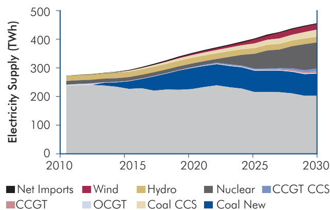
Figure 3.2: Electricity Generation for Southern African Region—Baseline Scenario
