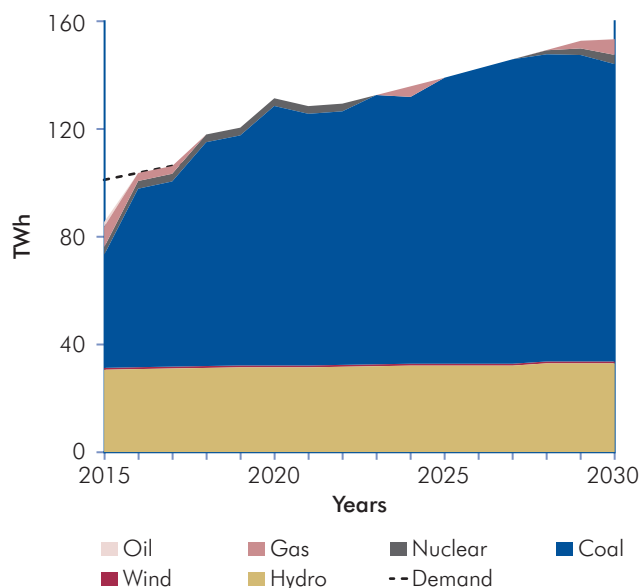
Figure 3.8: Electricity Generation for the Balkan Region—Reference Scenario
