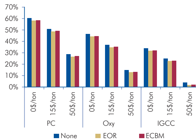
Figure E.1: Percentage Change in LCOE from Reference Plant without CCS to Plant with CCS with Enhanced Hydrocarbon Recovery and CO 2 Price
