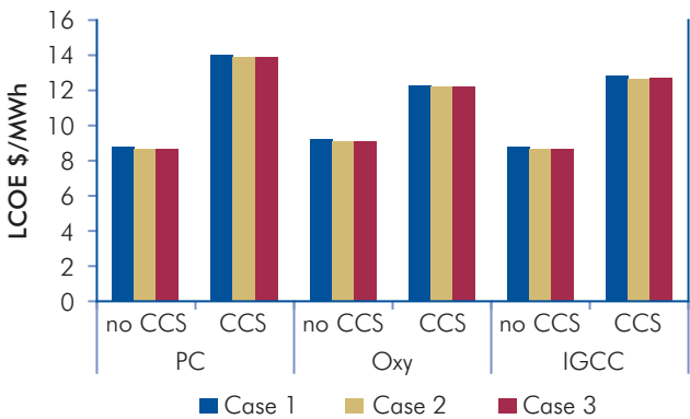
Figure 6.6: LCOE Variations with Different Financial Structures
