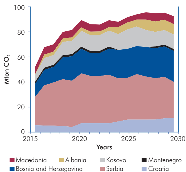
Figure 3.9: CO 2 Emissions for the Balkan Region—Reference Scenario
