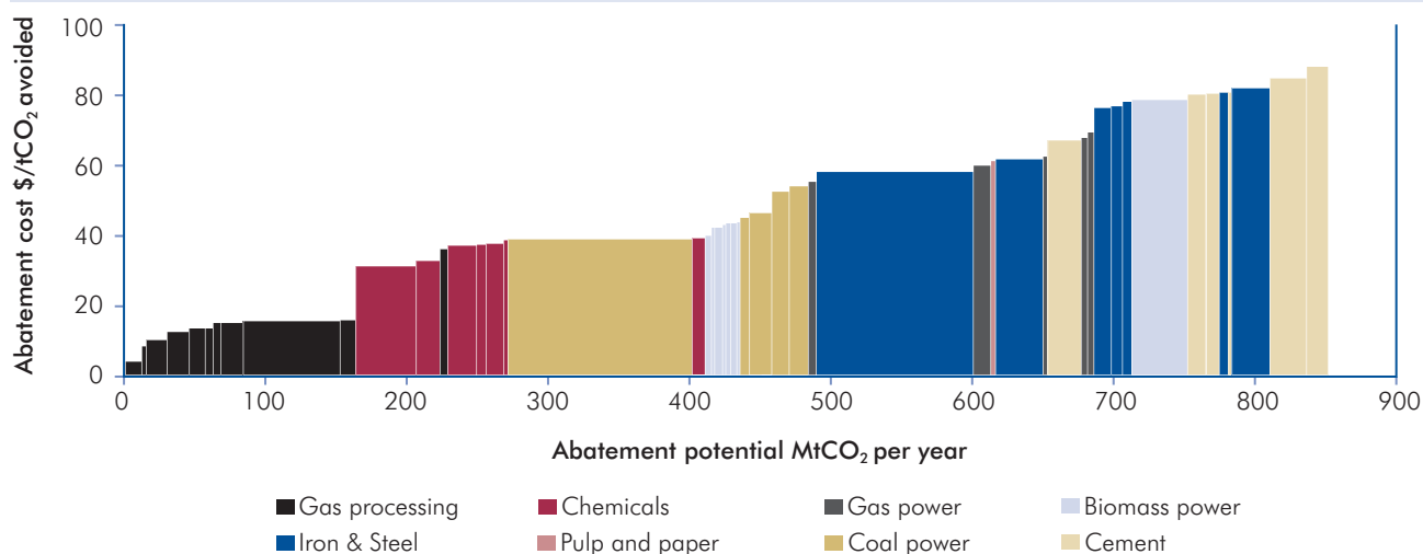
Figure 5.2: Marginal Abatement Cost Curves for CCS in 2030 by Sector and Region
