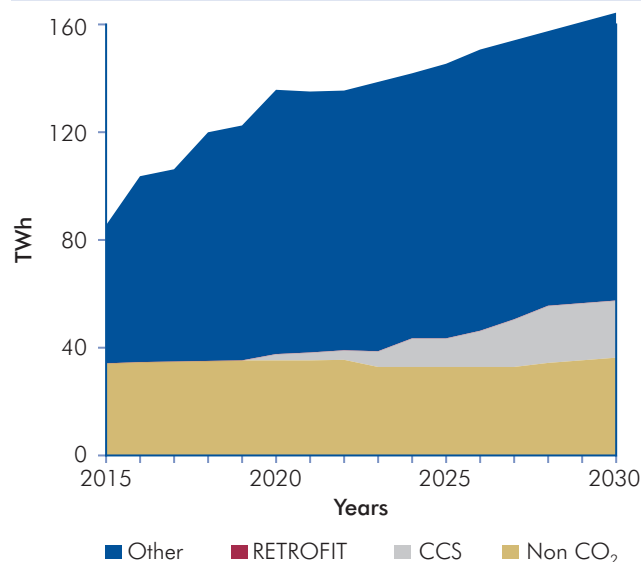
Figure 3.10: Share of CCS in Coal-Based Power Generation in the Balkan Region—Reference Scenario with EOR/ECBM benefits
