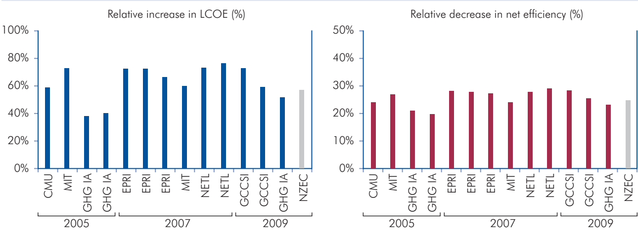
Figure 2.2: Comparison of Studies of LCOE Increase and Net Efficiency Decrease for Post-Combustion Power Plants with CCS
