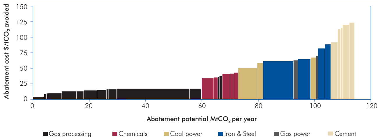
Figure 5.1: Marginal Abatement Cost Curves for CCS in 2020 by Sector and Region
