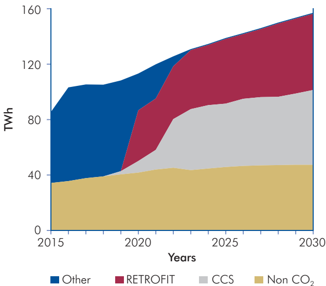
Figure 3.11: Share of CCS-Based Generation in the Balkan Region—US$100/Ton CO 2 Price Scenario
