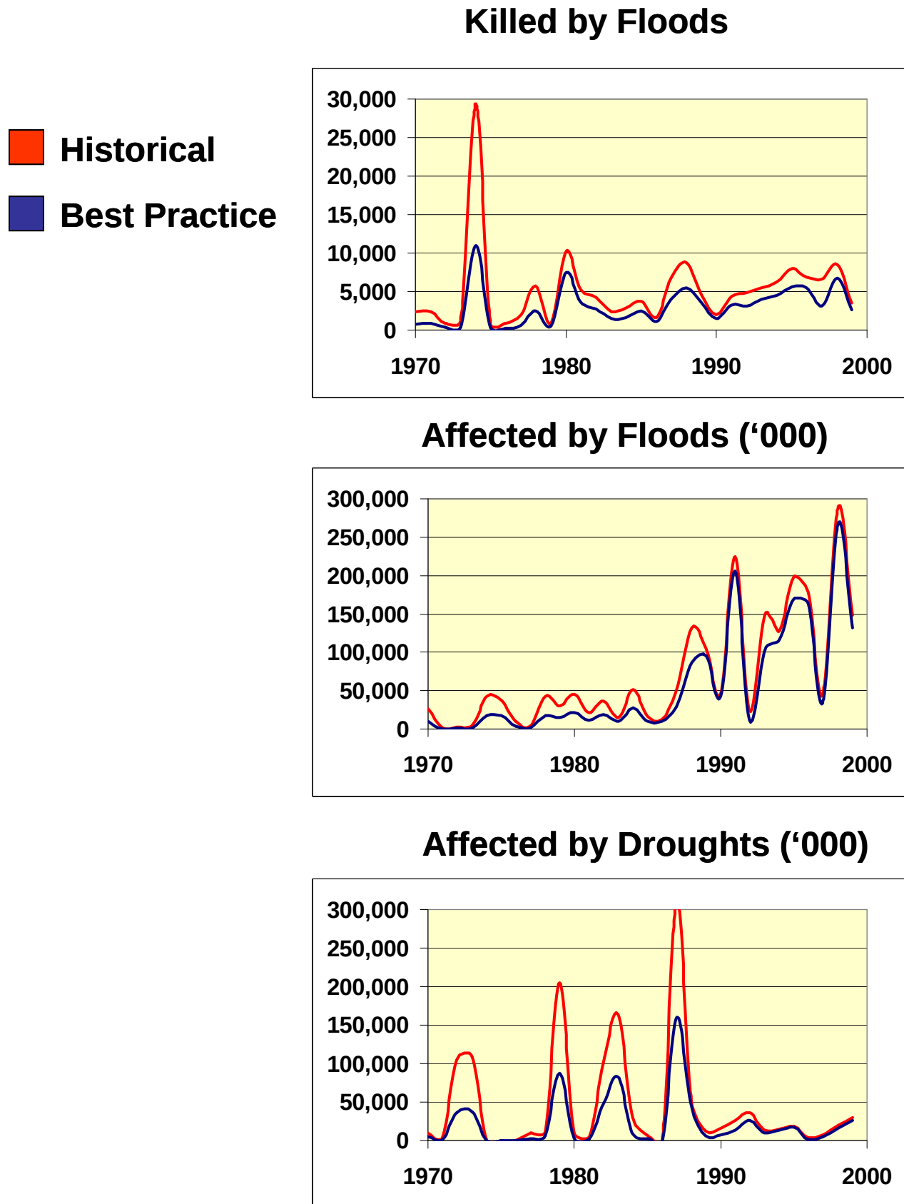
Figure 4: Extreme Weather Losses, 1970-1999 Historical and Best Practice
