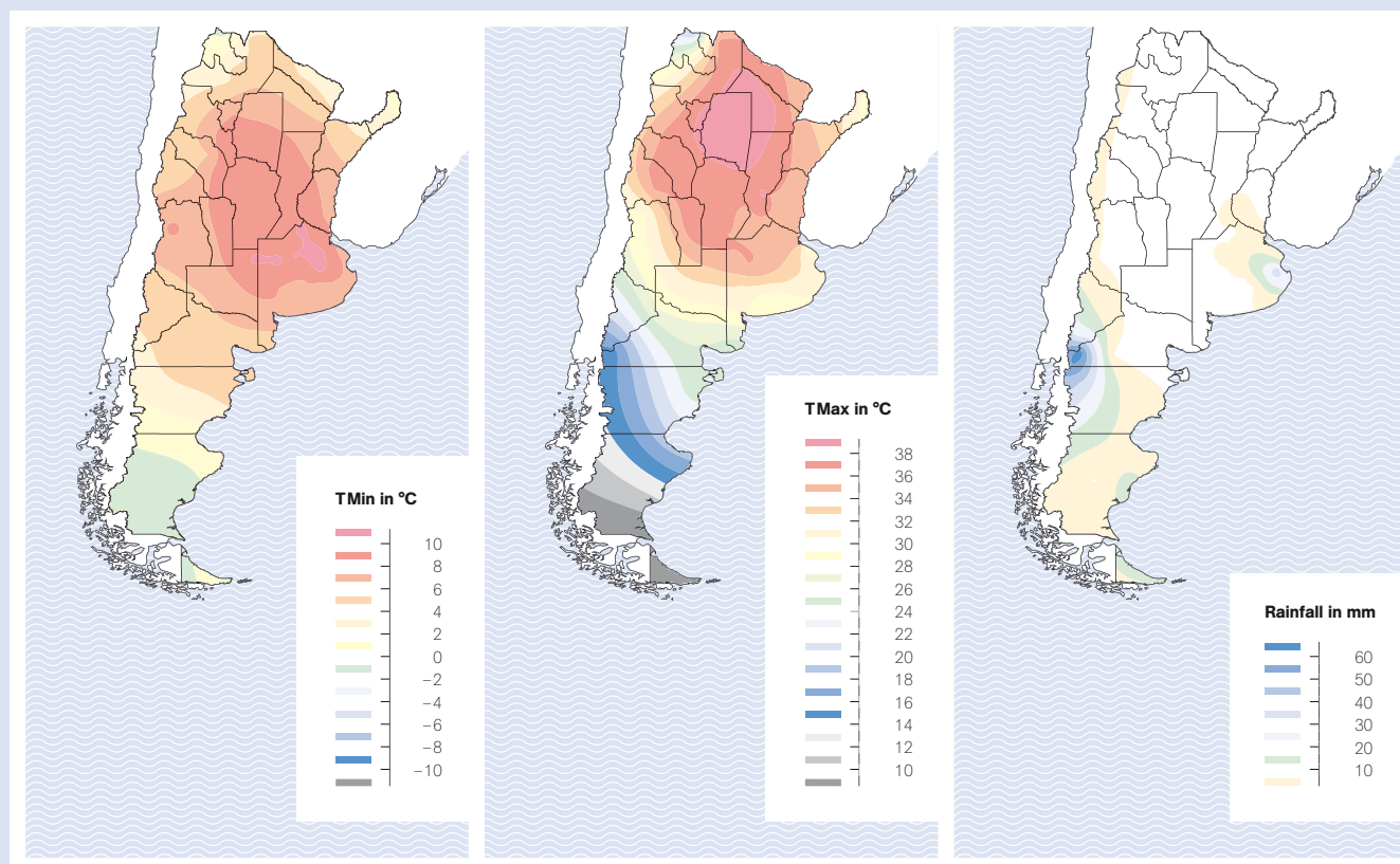
Figure II-3. Examples of weekly forecasts of temperature and rainfall
