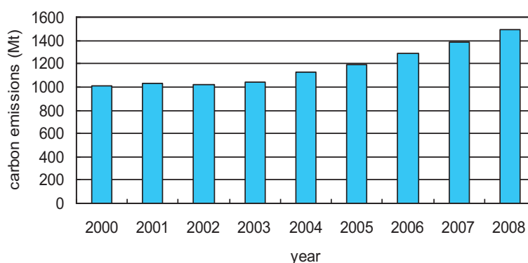
Figure 3-34. CO 2 emission in India from 2000 to 2008
