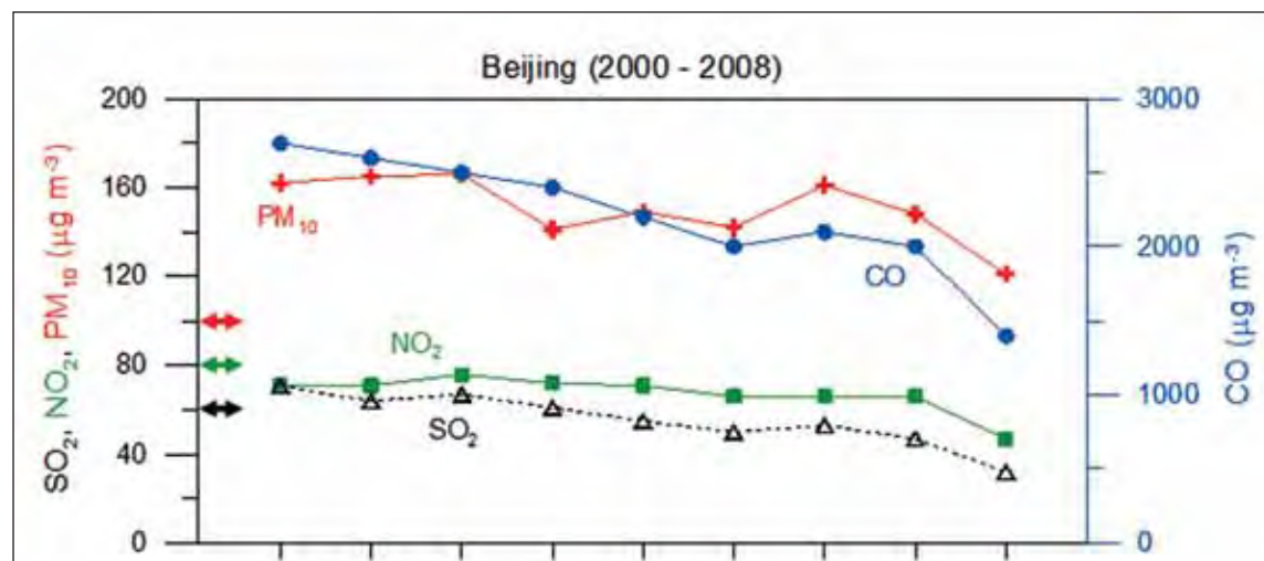
FIGURE 2.1: NETWORK-AVERAGE ANNUAL MEAN CONCENTRATIONS OF THE MAIN POLLUTANTS IN BEIJING, 2000 – 2008
