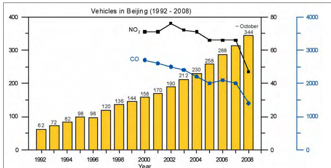
FIGURE 3.1: NUMBER OF VEHICLES AND NO 2 AND CO CONCENTRATIONS IN BEIJING, 1992-2008
