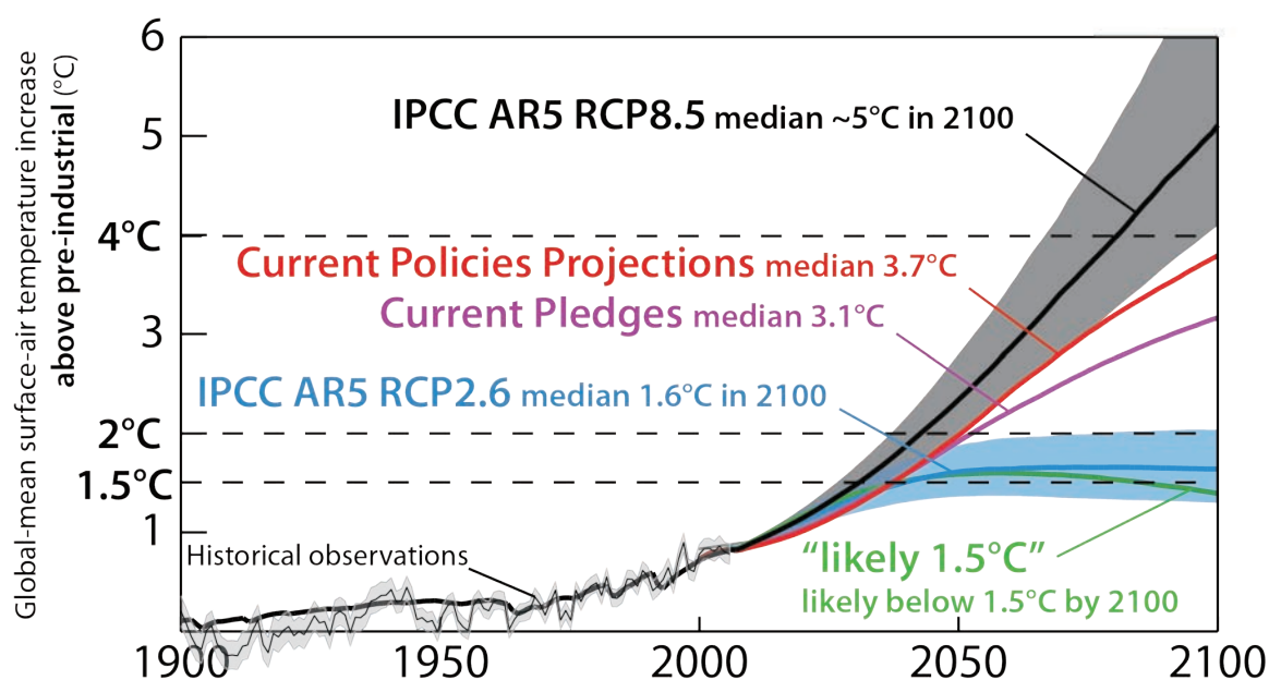
Figure 1- Projections for global-mean surface-air temperature increase, showing the scenarios assessed in this report. Lines indicate median estimates and colored areas uncertainty ranges driven by climate-system, as well as carbon-cycle processes (only shown for RCPs for clarity). Methods as in Schellnhuber et al (2014).
