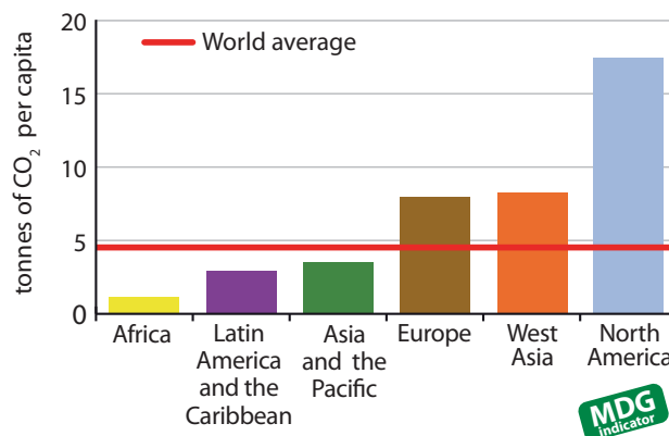
Figure 3: Carbon dioxide emissions per capita, 2008. Per capita emissions of CO 2 are well above the global average in Europe, West Asia and, most notably, North America. Source: GEO Data Portal, compiled from Boden et al. (2011)
