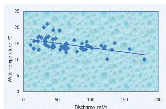
Figure 26. Relationship between discharge (river gauging station at Zaisan) and water temperature (at Ulaanbaatar meteorological station) in month of July (1978-2008)
