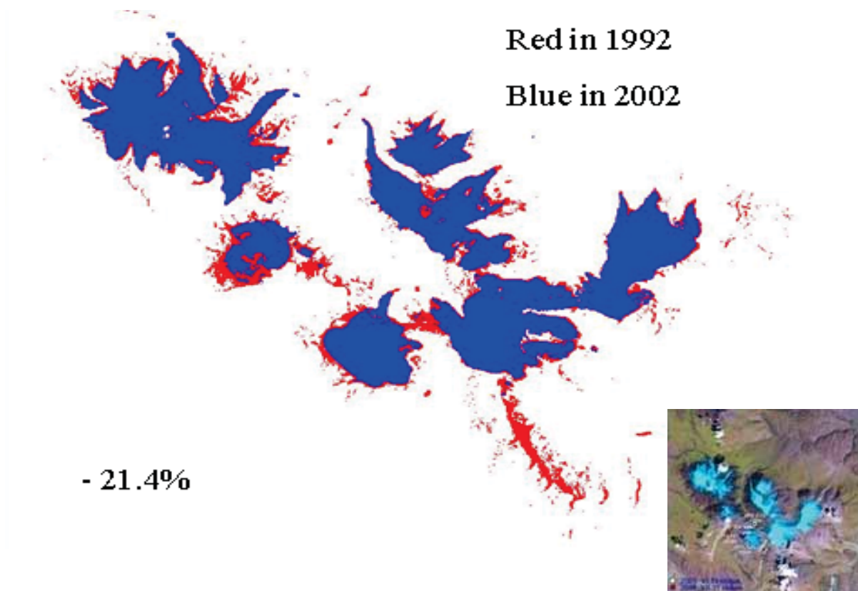
Figure 8. Glacier changes between 1992-2002 at Tsambagarav mountain in Mongolia (Source: Davaa et. al., 2008)
