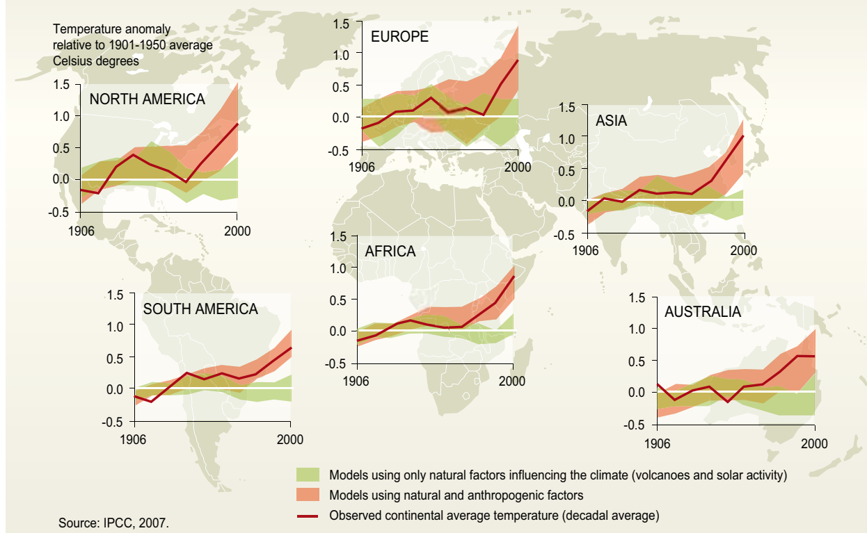
Observed and modelled temperature change between 1906 and 2005
