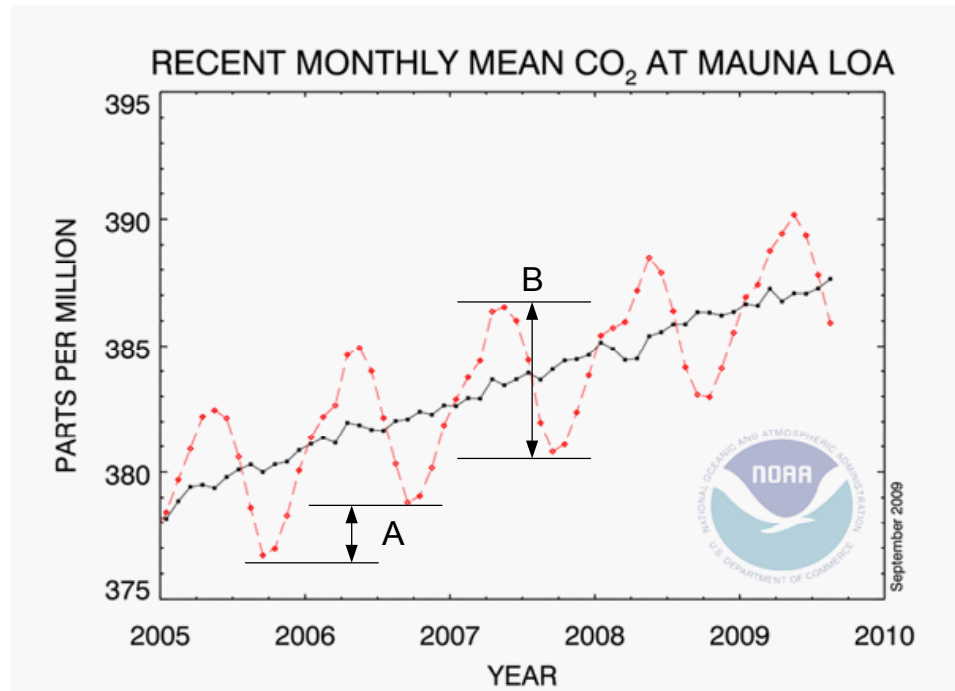
Figure 2. Mean monthly CO 2 concentration cycles at Mauna Loa, Hawaii showing seasonal patterns (red line) and trend from moving average corrected for the seasonal cycle (black line). Mean monthly data source: NOAA ( http://www.esrl.noaa.gov/gmd/ccgg/trends/ ).
