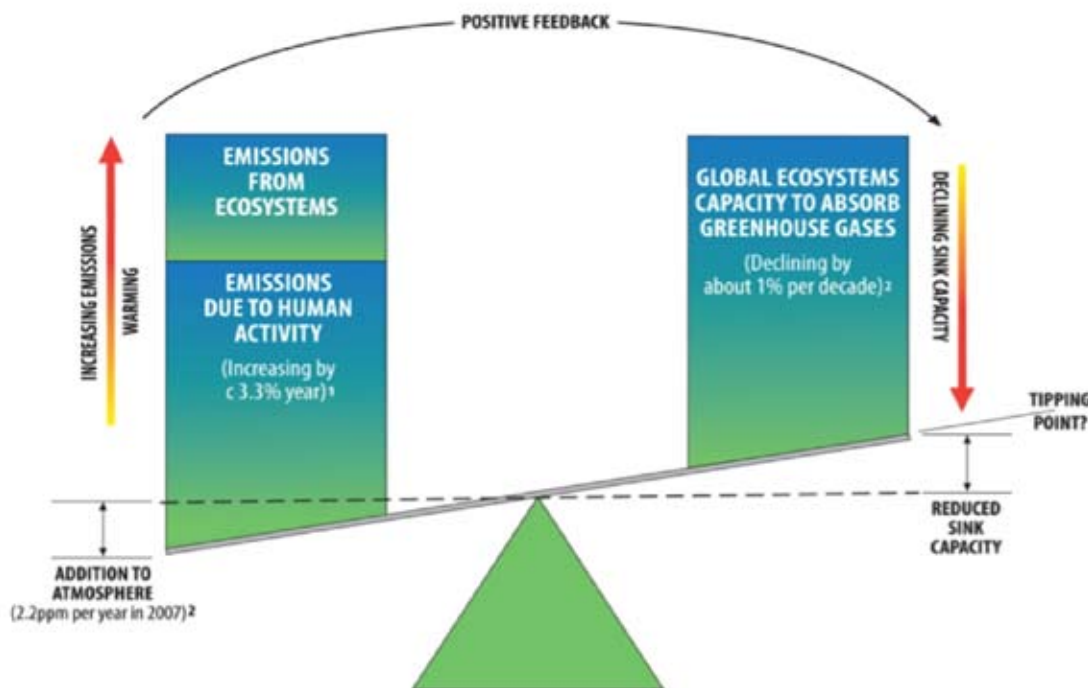
Figure 1. Imbalance of components for climate stabilisation Global Carbon Budget 13 (Note proportions of size are not to scale and do not reflect actual values of fluxes)
