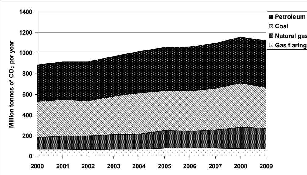
Figure 6 CO 2 emissions from the consumption of fossil fuels in Africa 2000 - 2009 Source: EIA (2011)
