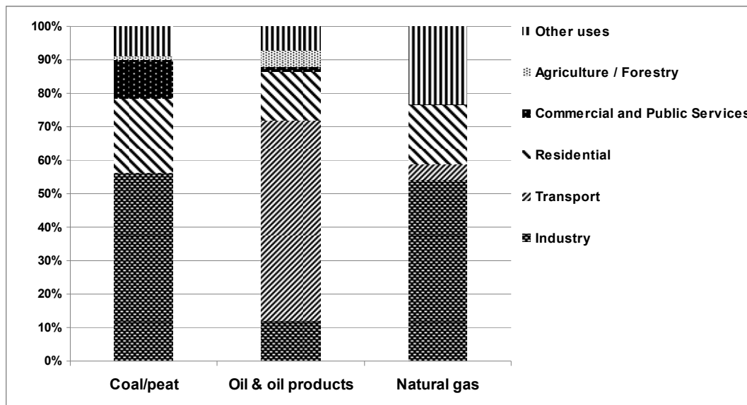
Figure 5 Sectoral consumption of fossil fuels in 2008 Source: IEA (2011a)
