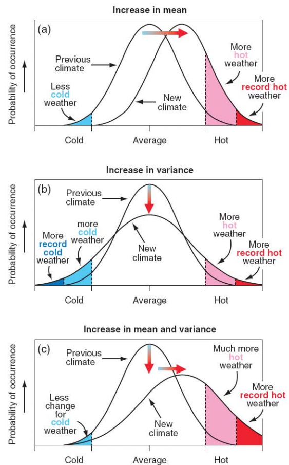
Figure 1.4 Climate Change Alters the Distribution of Weather Events
