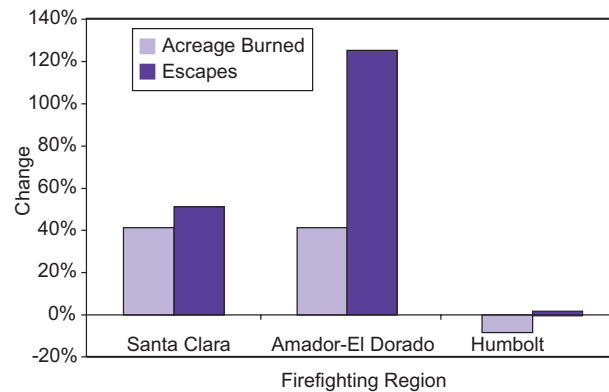
Figure 2.26 Rising CO 2 and Wildfires
