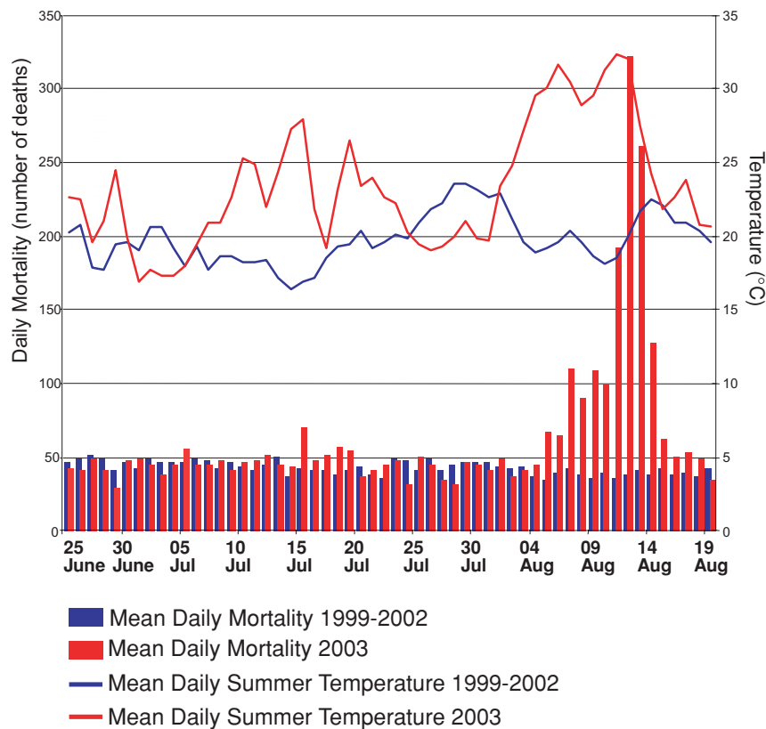
Figure 2.19 The Paris Heat Wave: Deaths and Temperatures
