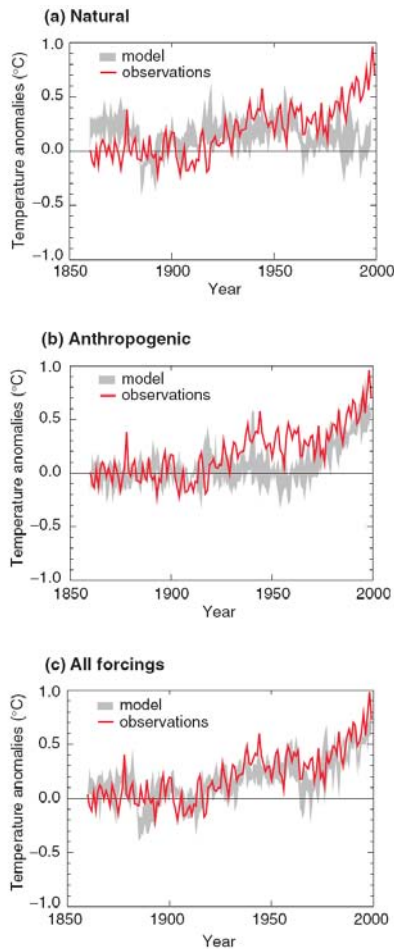
Figure 1.1 Simulated Annual Global Mean Surface Temperatures
