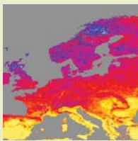
Temperatures in 2003 were 10°C (18°F) above long-term Summer averages Image – NASA/Earth Observatory
