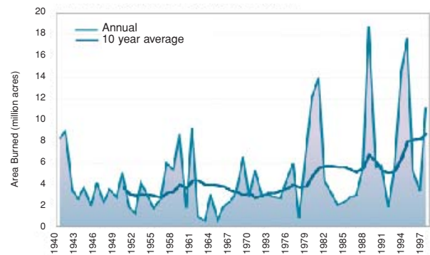
Figure 2.25 Annual Area of Northern Boreal Forest Burned in North America
