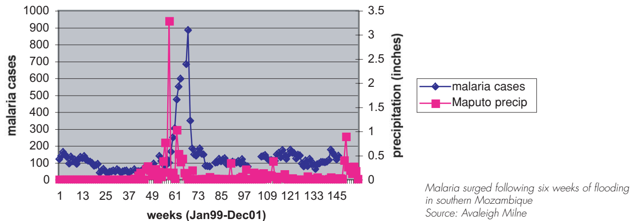
Figure 2.4 Malaria and Floods in Mozambique
