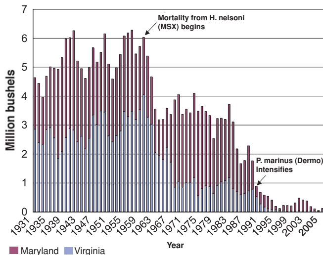
Figure 2.34 Chesapeake Bay Market Oyster Landings: 1931-2005
