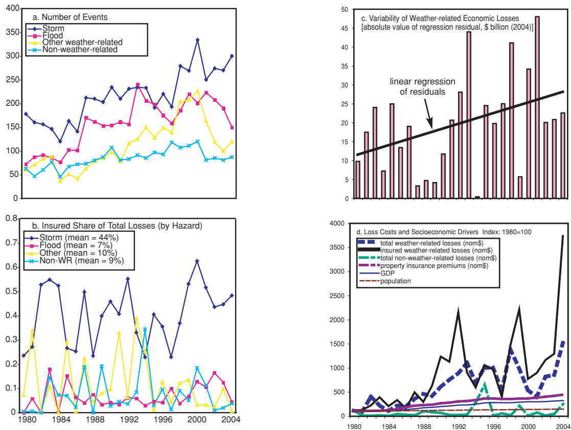
Figure 1.7 Trends in Events, Losses and Variability: 1980-2004
