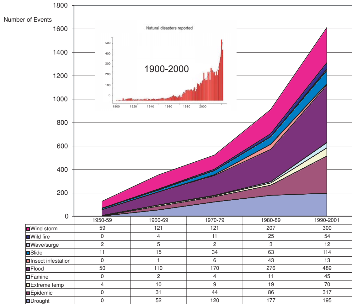
Figure 1.6 The Frequency of Weather-Related Disasters
