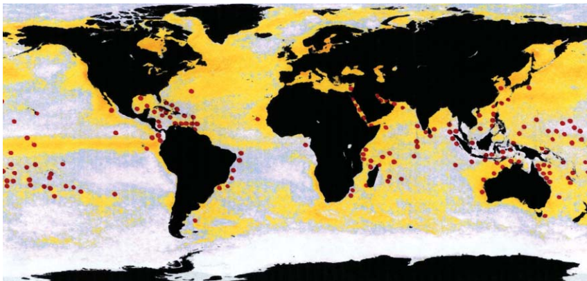
Figure 2.31 Sea Surface Temperatures and Coral Bleaching
