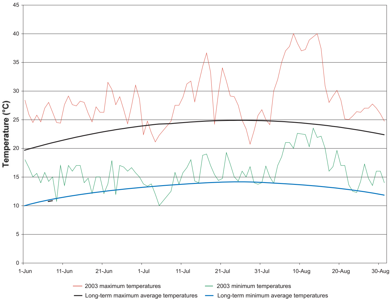
Figure 2.18 Paris Temperatures in Summer 2003
