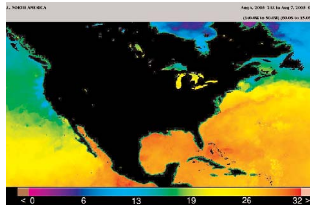
Figure 1.2 The Warming Tropical Seas
