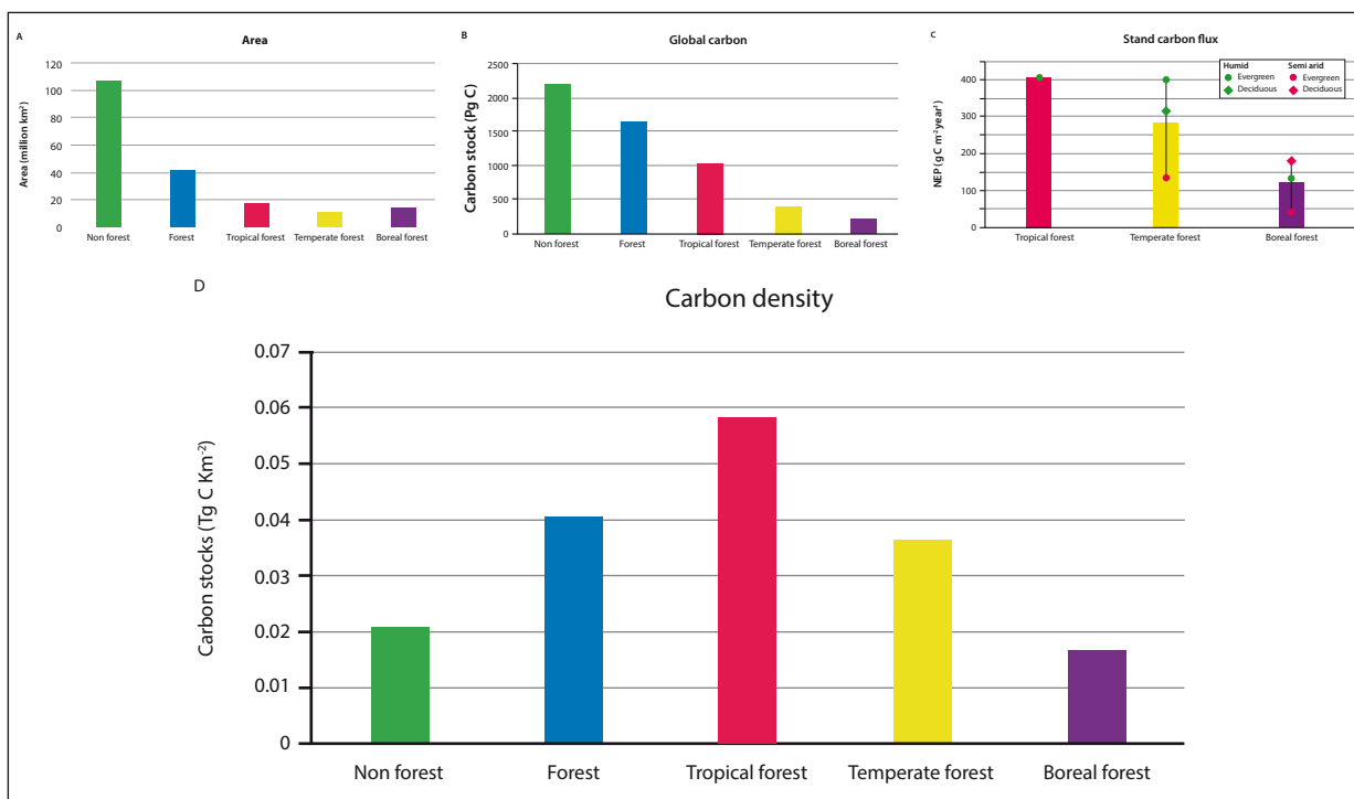
Figure 2. Forests and Carbon. (A and B) Current extent and total (above and below ground) terrestrial carbon storage for forest and non-forest, and biomes. (C) Stand level NEP by biome. Tropical forests have relatively higher rates of carbon sequestration. (D) Carbon Density. Forests generally hold proportionally greater quantities of carbon per unit area than non-forests; Tropical forests store more carbon per unit area than do Temperate or Boreal systems.
