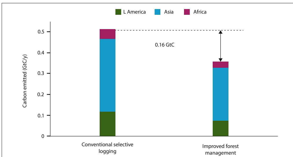
Figure 4.1: Annual Reductions in Global Carbon Emissions that Would Result from Adoption of Improved Tropical Forest Management Practices (Protocol S1)
