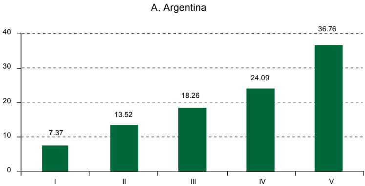
Figure 12 Proportion of total expenditure on food and beverages represented by household expenditure on food and beverages, by income quintile (Percentages)
