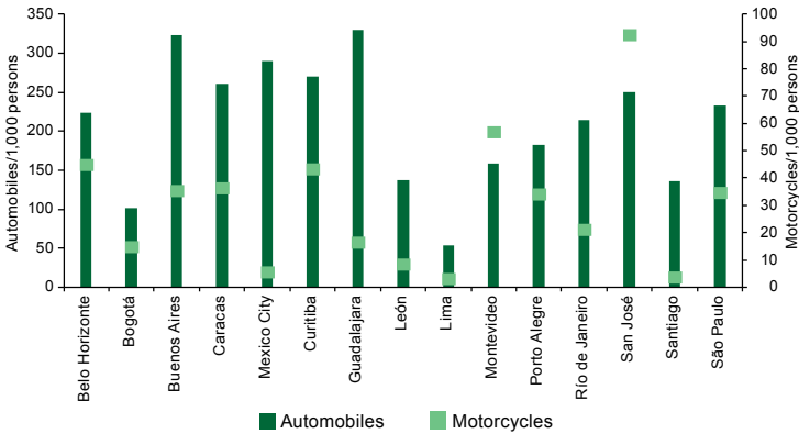
Figure 17 Rate of motor vehicle use in selected Latin American cities, 2007 (Automobiles and motorcycles per 1,000 persons)
