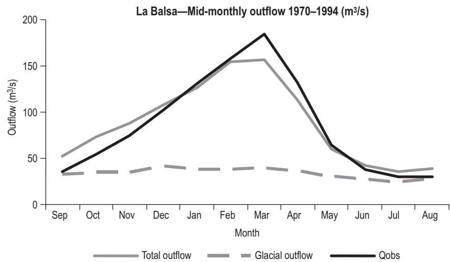
Figure A4.13. Mid-monthly calculated and simulated streamflows ( m^3/s ) for three watersheds, 1969–1997
