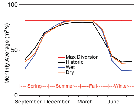
Figure 6.3. Flow through Cañón del Pato for historical conditions, marginally warmer and much warmer scenarios
