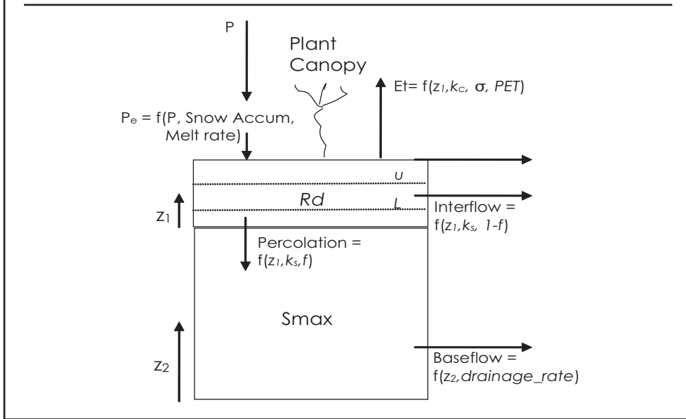
Figure A4.9. Schematic of the two-layer soil moisture store, showing the different hydrologic inputs and outputs for a given land cover
