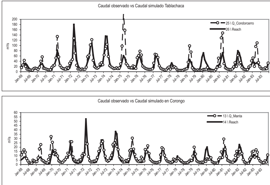
Figure 5.1. Calibration and validation of model in the Corongo Basin for two historical periods: 1967–1983 and 1984–1999
