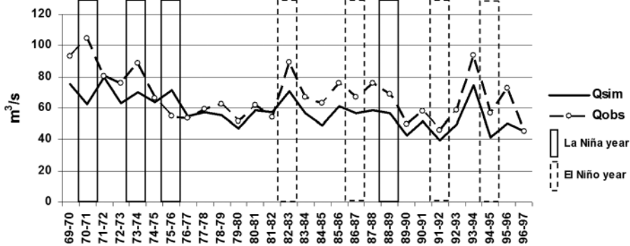
Figure A7.3b Interannual variability of simulated and observed streamflow at La Balsa gauge station between hydrologic years 1969–1970 and 1996–1997
