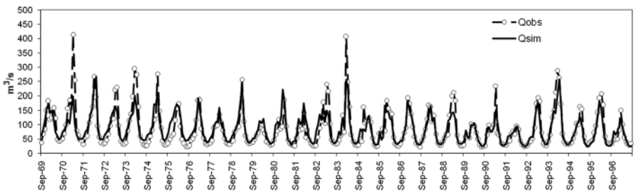
Figure A4.12. Correspondence between simulated (continuous thick line) and observed (broken thick line) streamflow at La Balsa gauge station between September 1969 and August 1997
