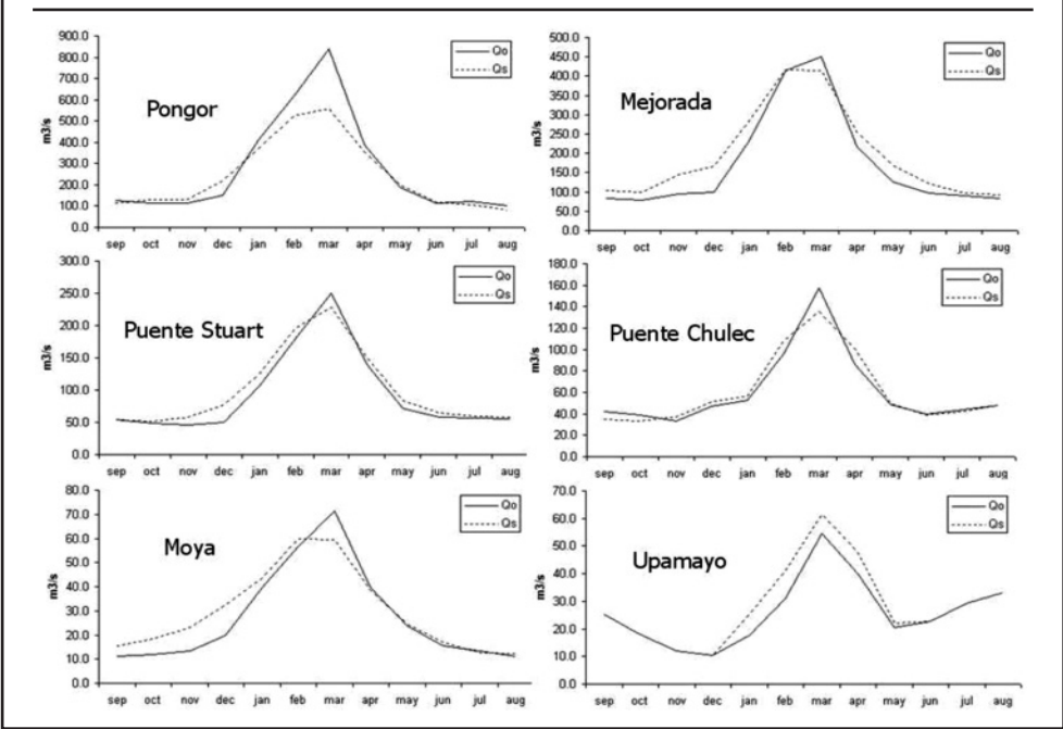
Figure 5.7. Observed ( Q_o ) and simulated ( Q_s ) monthly average streamflows for the Mantaro River Basin during the 1970–1981 calibration period
