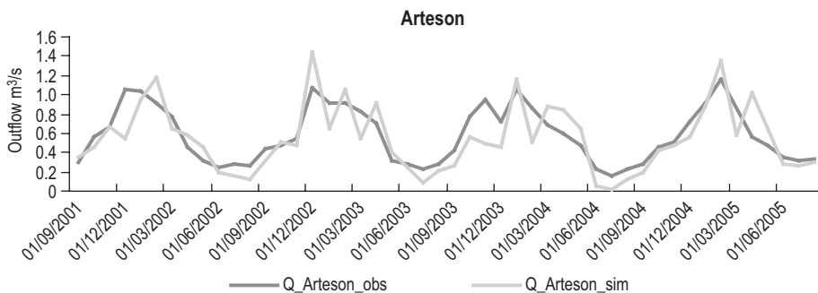
Figure A4.11. Outflow at Artesoncocha gauge station: comparison between observed and simulated values between September 2001 and August 2005, R^2=0.67 p \leq 0.05
