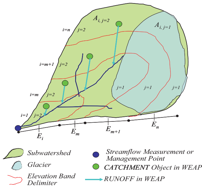
Figure 4.1. Illustration of sub-basins and elevation bands
