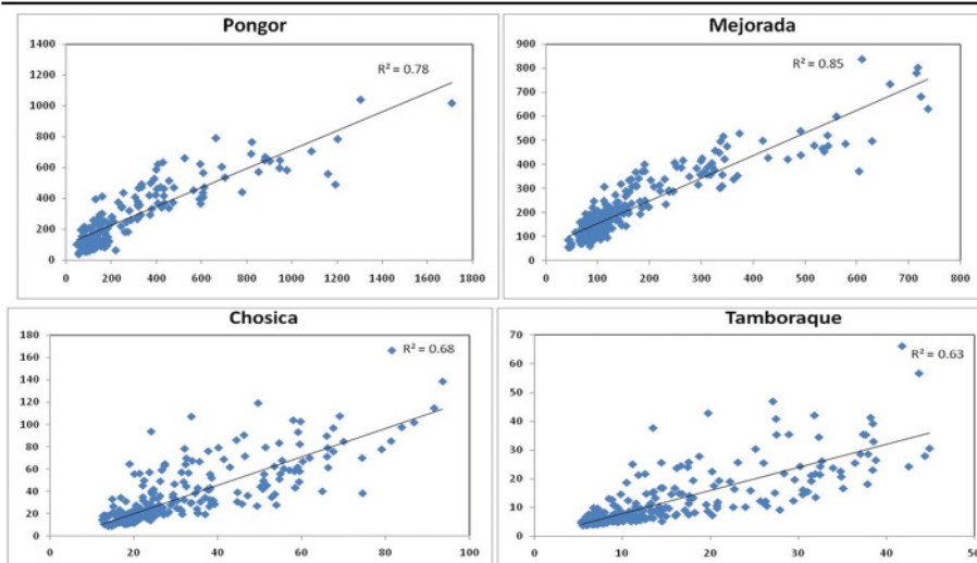
Figure 5.9. Correlation between observed and simulated flow rates for the reference period
