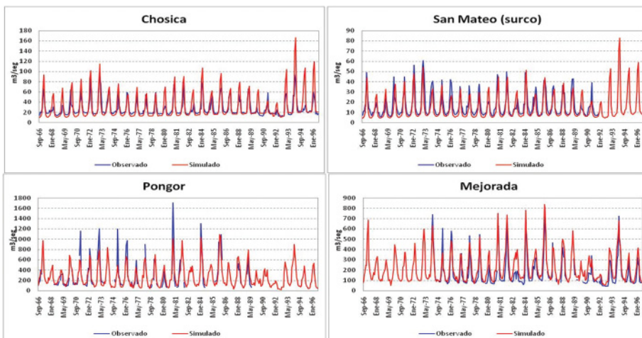
Figure 6.7. Observed (blue line) and projected (red line) discharges using trend analysis at selected sites on the Rímac and Mantaro Rivers, 1966–1996
