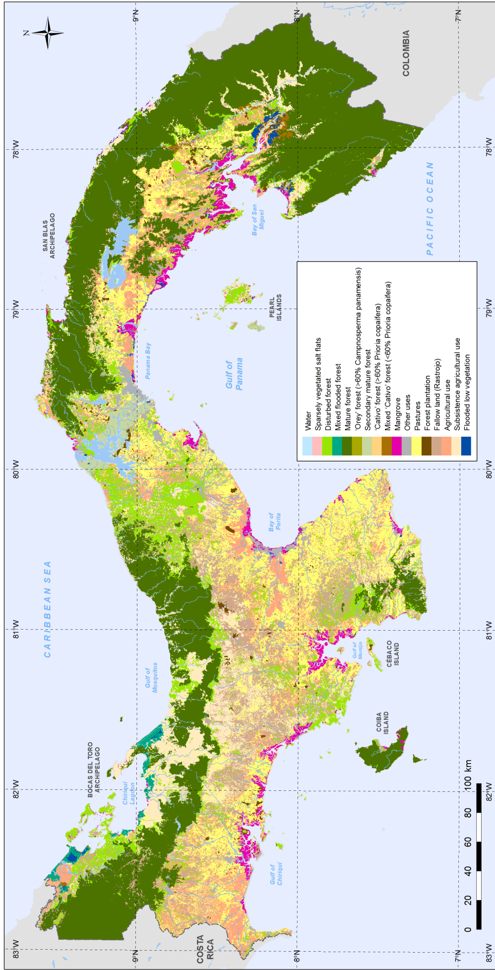
Map 1. Forest cover and land use
