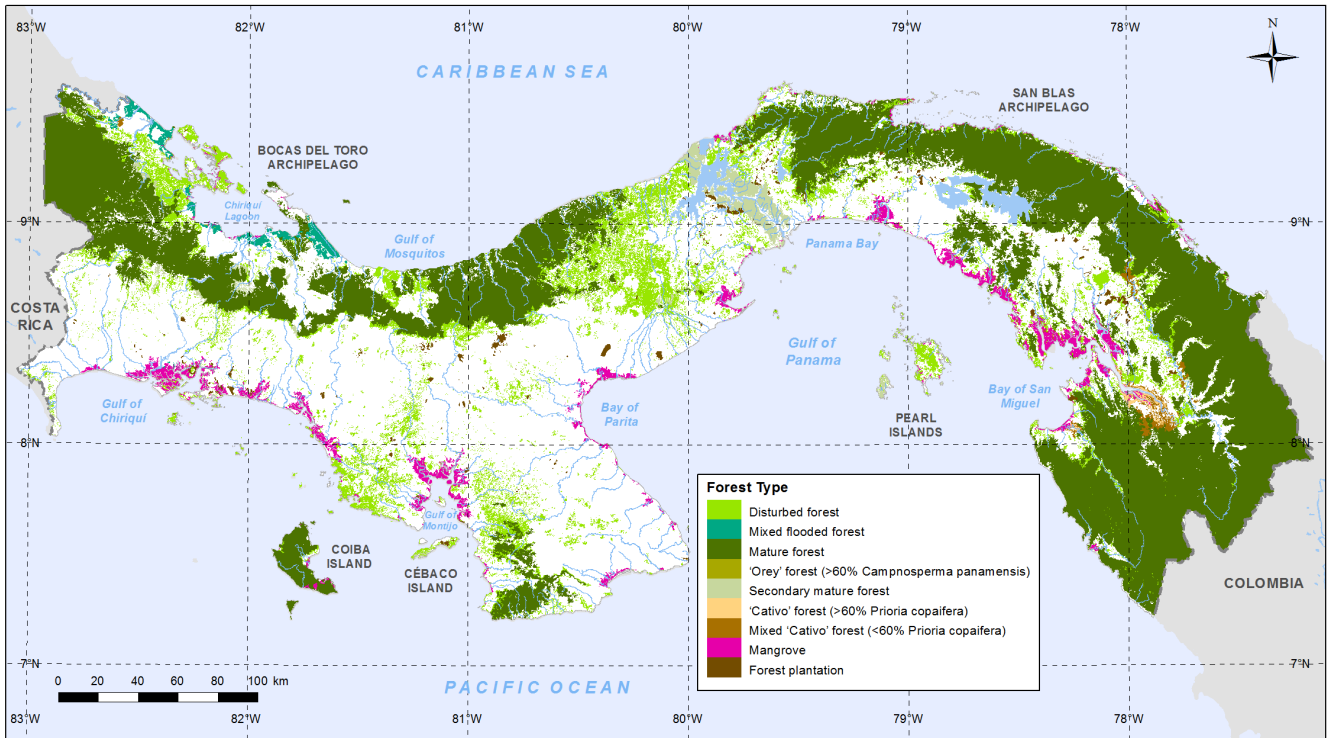
Map 2a. Forest cover showing major forest types An estimated 40–45% of Panama is currently forested.
