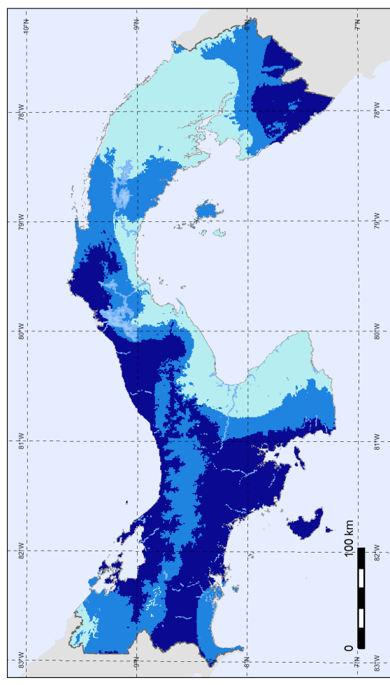
3 precipitation classes (May - Aug ~mm)
