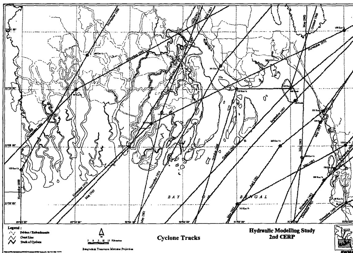
Figure 2.3: Path of Cyclones in Bangladesh
