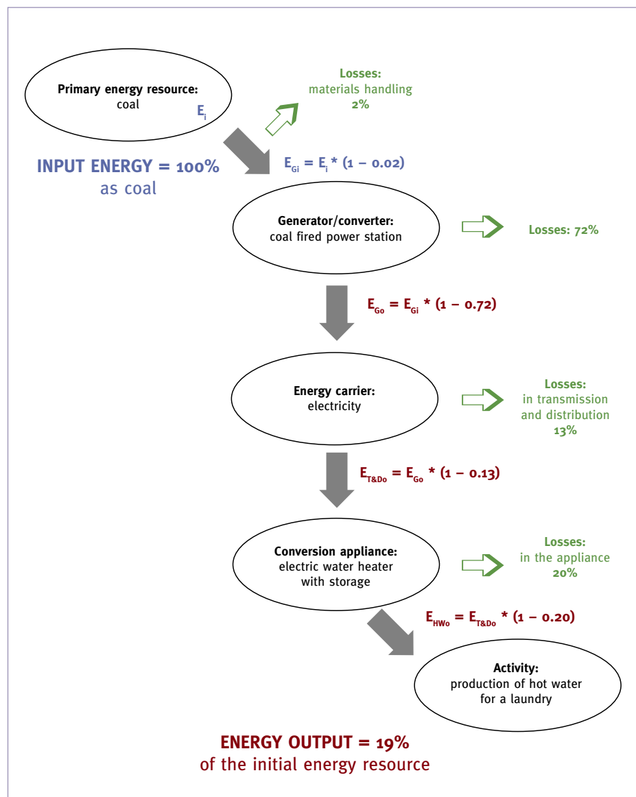
Figure III. Example of energy losses in hot water production
