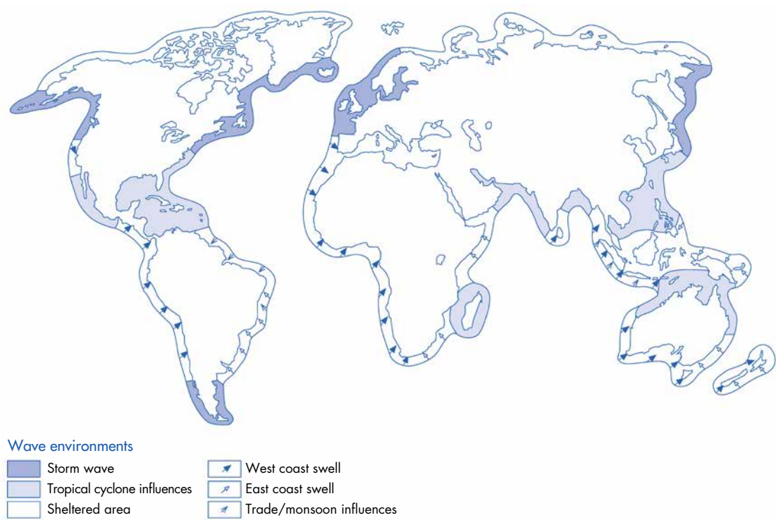
Fig. 4. Global wave environments (Davies 1980, modified by Masselink and Hughes 2003 and Rosendahl Appelquist).
