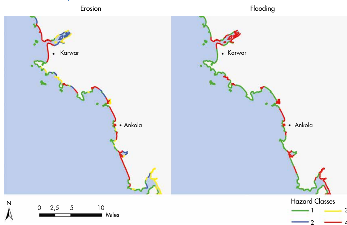
Fig. 30. Sub-regional hazard maps for northern Karnataka, India showing the hazards of erosion and flooding (Rosendahl Appelquist and Balstrøm 2015).
