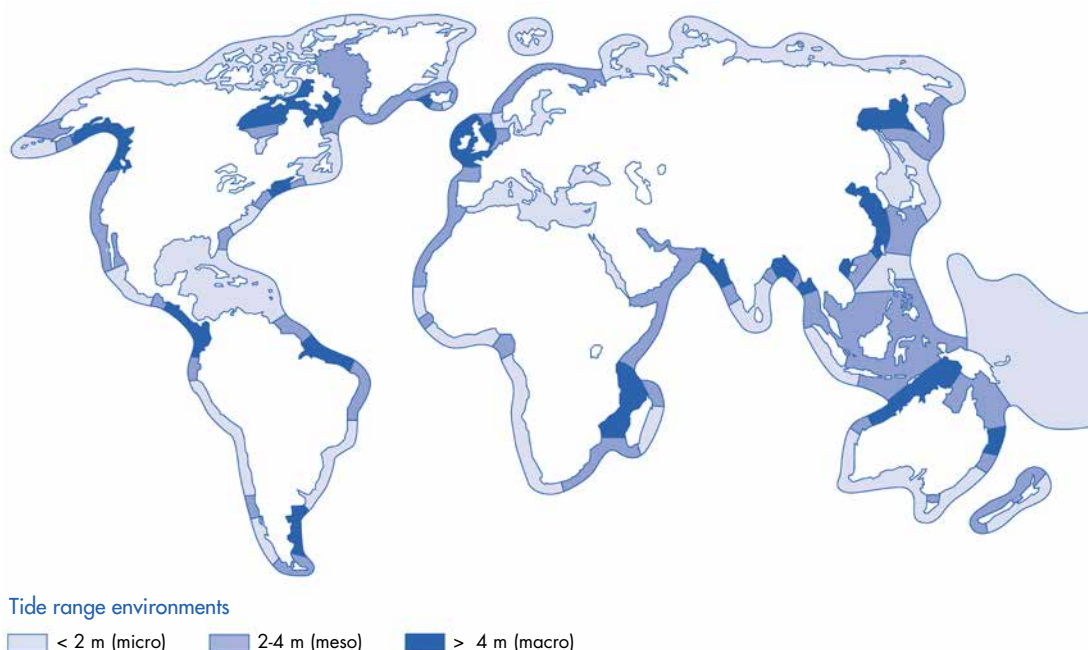
Fig. 5. Map over global tidal environments (Davies 1980, modified by Masselink and Hughes 2003).
