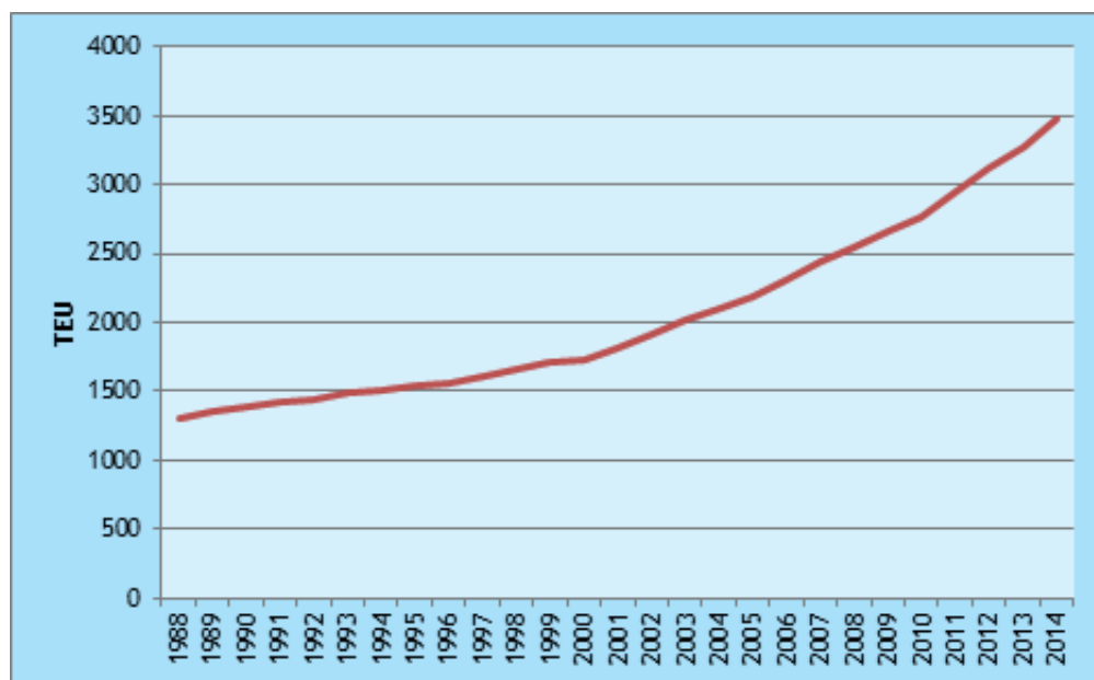
Figure 43: Historical development of average ship size of cellular fleet
