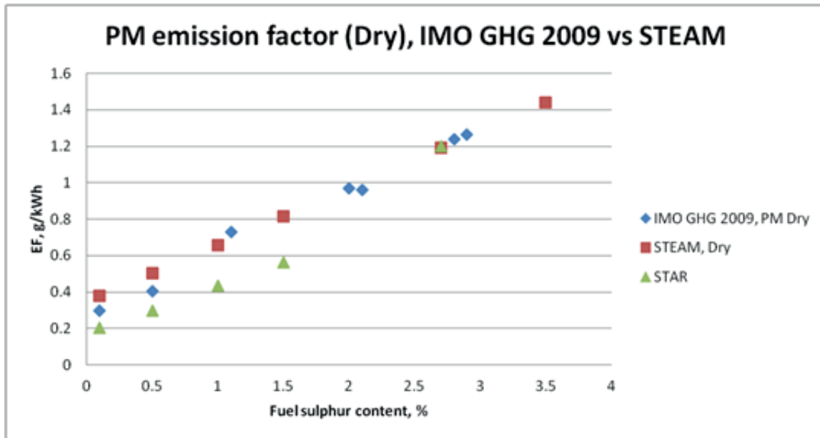
Figure 74: Comparison of PM emissions factors reported in Second IMO GHG Study 2009 [blue diamond] (Figure 7.7, based on data from Germanischer Lloyd) with values from Jalkanen et al. (2012) [red square] and Starcrest (2013) [green triangle]
