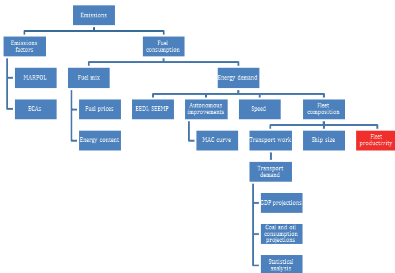
Figure 36: The role of fleet productivity in the model structure
