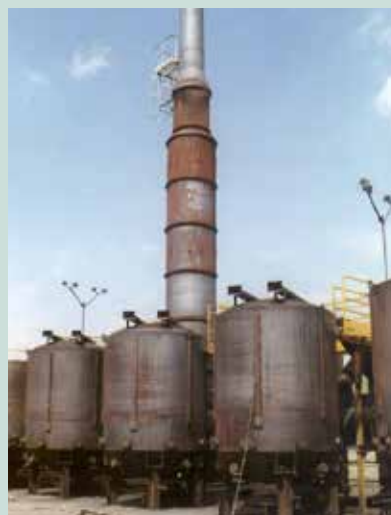
Metal kilns equipped with vapour incinerator for charcoal production in France
