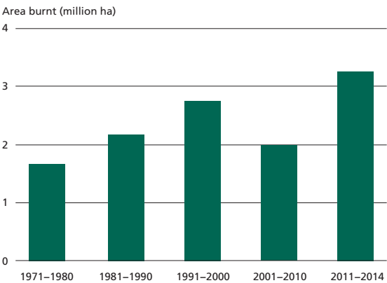
FIGURE 20 Decadal forest areas burnt in Canada, 1971–2014
