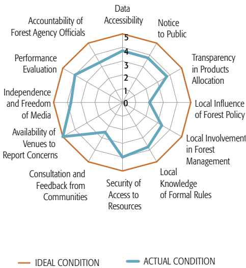
FIGURE 6: RESULTS FROM SCORING INDICATORS IN UGANDA PRESENTED IN A RADAR GRAPH
