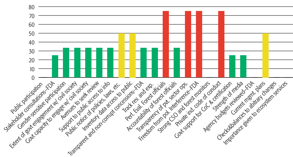
FIGURE 5: USING COLOR IN A BAR GRAPH TO DISPLAY INDICATOR SCORES FROM LIBERIA
