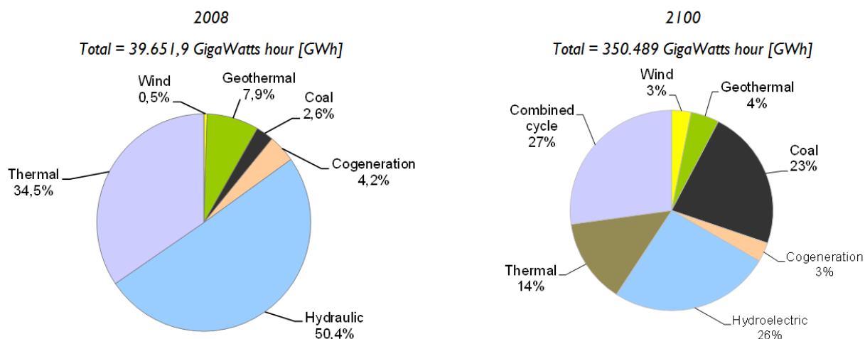
CHART 28 CENTRAL AMERICA: ELECTRICITY GENERATION, BY TYPE OF TECHNOLOGY WITH BASELINE SCNEARIO IN 2100
