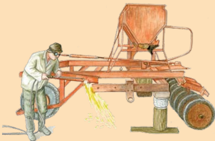
Kazakhstani farmers have modified traditional wheat plough-seeders to enable direct-seeding through residues, without tillage
