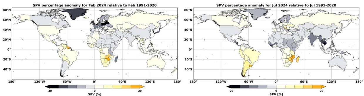
Figure 5. As in Figure 4, but for February (left) and July (right) 2024, relative to their average corresponding month in the period 1991–2020. Note the range of values is twice that of the annual mean.
