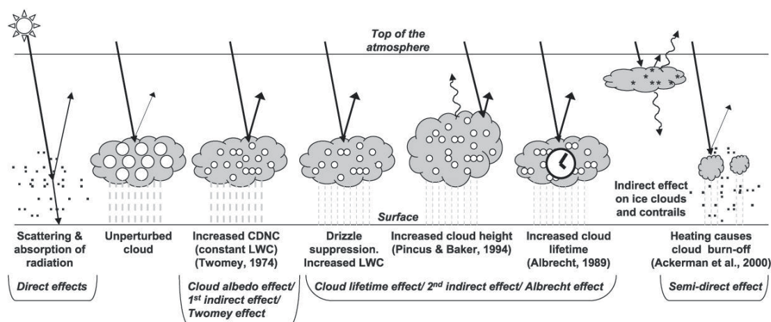
Figure 5.18. Schematic diagram showing the major radiative forcing mechanisms related to aerosols. The small black dots represent aerosol particles; the larger open circles cloud droplets. Straight lines represent the incident and reflected solar radiation, and wavy lines represent terrestrial radiation. The filled white circles indicate cloud droplet number concentration (CDNC). The unperturbed cloud contains larger cloud drops as only natural aerosols are available as cloud condensation nuclei, while the perturbed cloud contains a greater number of smaller cloud drops as both natural and anthropogenic aerosols are available as cloud condensation nuclei (CCN). The vertical grey dashes represent rainfall, and LWC refers to the liquid water content. [Adapted from Forster, P., et al. (2007), Changes in atmospheric constituents and radiative forcing, Climate Change 2007: The Physical Scientific Basis , Cambridge University Press, Cambridge, United Kingdom and New York, NY, USA.]
