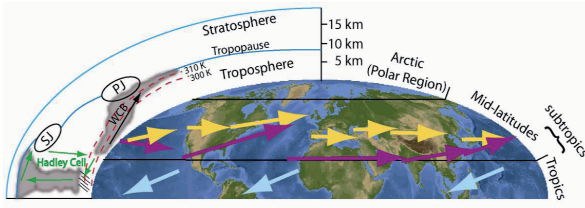
Figure 1.7. Schematic diagram showing some of the main features of the atmosphere related to the transport of air pollutants. The vertical cross section shows the average location of the tropopause (the boundary between the troposphere and stratosphere) and the polar (PJ) and subtropical (SJ) jet streams during winter. Vertical transport during winter is dominated by deep convective clouds in the tropics (the upward branch of the Hadley cell) and WCBs in the mid-latitudes, as described in Section 1.3.2. The average location of the jet stream is shown across the entire Northern Hemisphere for winter (magenta arrows) and summer (yellow arrows); locations of the tropical easterlies are also shown (light blue arrows). Also shown are the winter locations of the 300 K and 310 K potential temperature surfaces (red).
