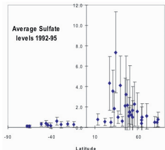
Figure 2.15. Average sulphate levels measured at marine sites in the Northern and Southern hemispheres [Barrie et al. , 2001].
