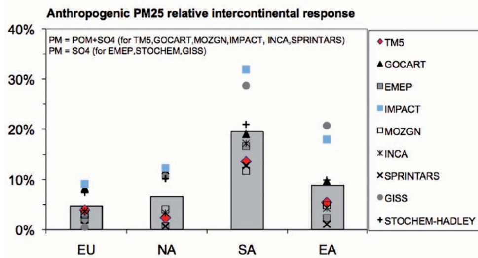
Figure 4.22. Relative annual intercontinental response of surface PM concentration over the HTAP regions (bars). Results from individual models are shown with symbols.
