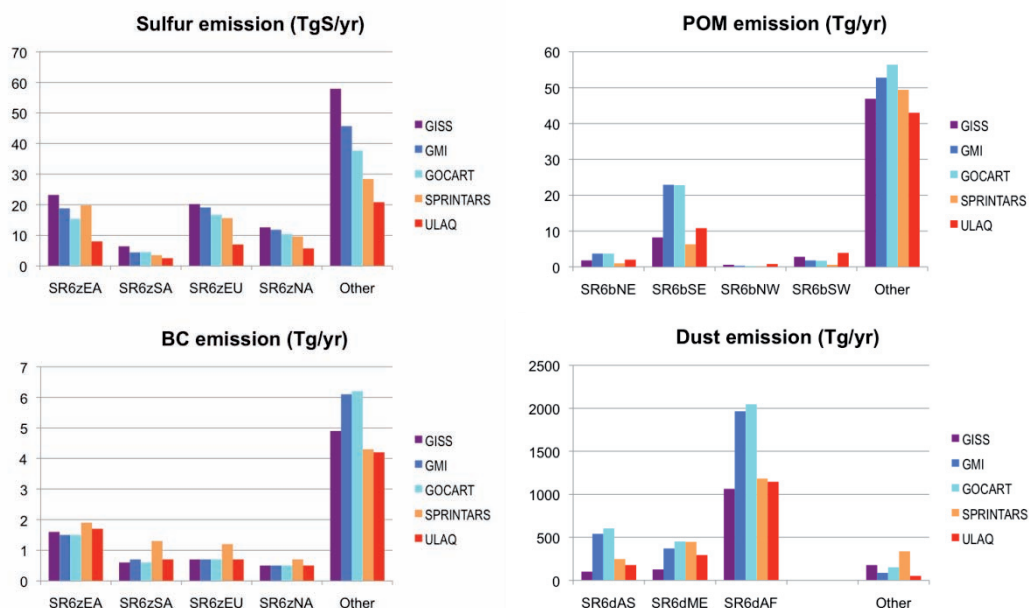
Figure 4.26. Emissions of anthropogenic sulphur (mostly \text{SO}_2 ) and BC in anthropogenic source regions, POM in biomass burning regions, and dust in desert regions. Emissions from other global regions are shown as “other”.
