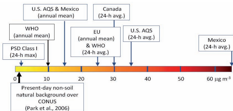
Figure 5.2. Current 24-hr. and annual mean PM 2.5 standards for selected countries, and U.S. allowable 24-hr emissions increment for Class I areas under the Prevention of Significant Deterioration rule (CONUS is the continental United States). [Reprinted with permission from Figure 3.4 in Global Sources of Local Pollution: an Assessment of Long-Range Transport of Key Air Pollutants to and from the United States (2010), by the National Academy of Sciences, Courtesy of the National Academies Press, Washington, D.C.]
