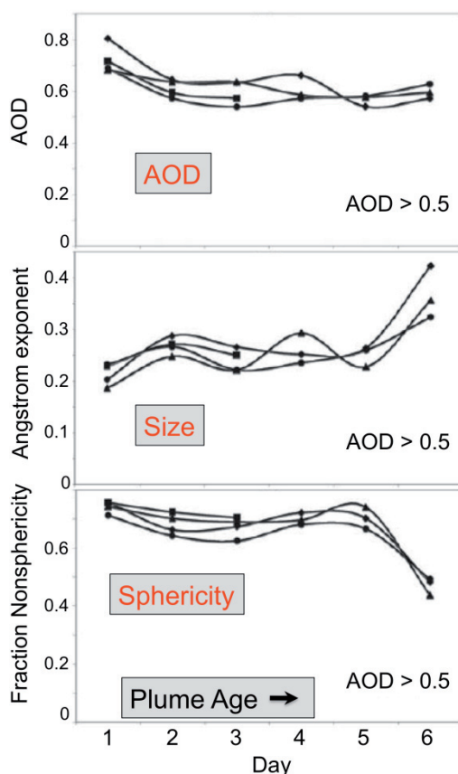
Figure 2.12. Evolution of dust plume characteristics for four case studies of dust transported from Africa to the Caribbean across the Atlantic in six days. Top: AOD, a total column measure of PM loading, decreases due to dry deposition. Center: Angstrom Exponent, an inverse measure of particle size. Particles on Day 6 are smaller than on Day 1 due to gravitational settling of the larger particles. Bottom: Particle sphericity showing less nonspherical fraction at the end of the transport due to increase in the hygroscopicity of particles and/or the removal of dust. [Reprinted from Figure 11 in Kalashnikova, O. V., and R. A. Kahn (2008), Mineral dust plume evolution over the Atlantic from MISR and MODIS aerosol retrievals, Journal of Geophysical Research , 113(D24204).]
