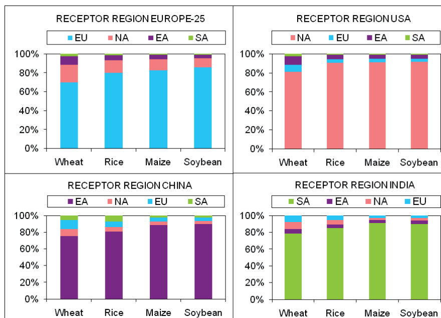
Figure 5.10. The relative contribution of each HTAP region to crop damage (expressed as relative yield loss) in each of 4 regions for run SR6 (20% decrease of O 3 and PM precursor emissions) using Mx and AOT40 indices.
