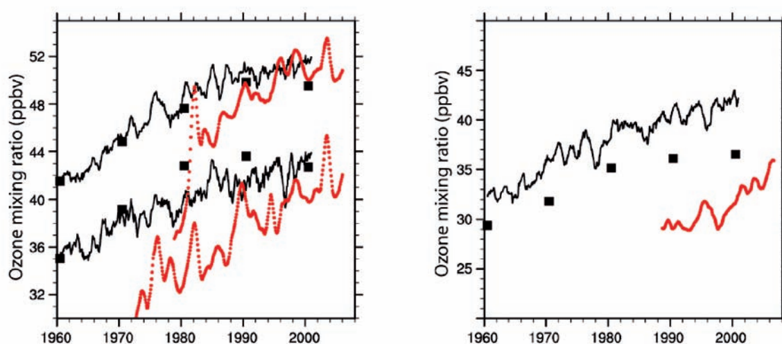
Figure 4.5. Comparison of surface O 3 trends (12-month running mean) from CAM-Chem (black line) and GISS-PUCCINI (black squares) against observations (red) at Zugspitze and Hohenpeissenberg, Germany (left) and US Pacific Coast sites (right). [Adapted from Figure 5 in Lamarque, J. F., et al. (2010), Historical (1850–2000) gridded anthropogenic and biomass burning emissions of reactive gases and aerosols: Methodology and application, Atmospheric Chemistry and Physics , 10: 7017–7039.]
